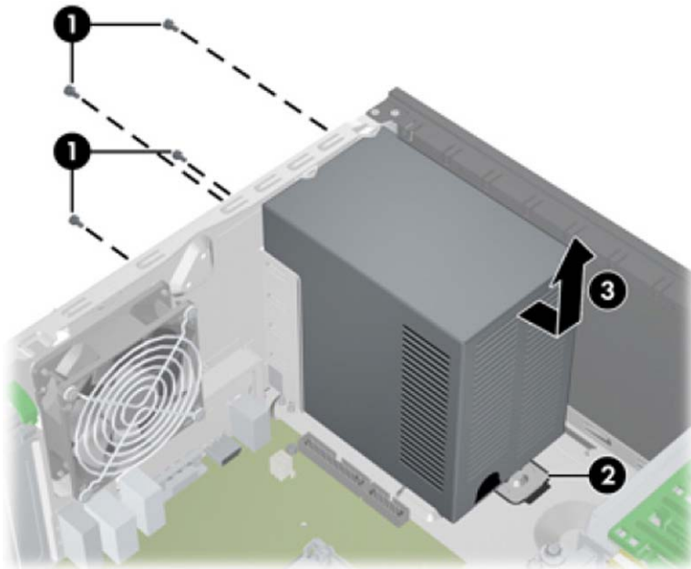
Figure 6-38 Removing the power supply
