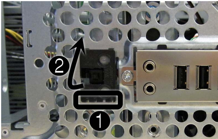
Figure 7-29 Removing the power switch/LED
