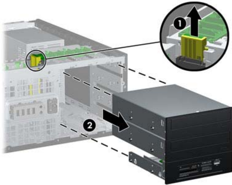
Figure 6-43 Releasing the 5.25-inch Drives from the Drive Bays (Desktop)
