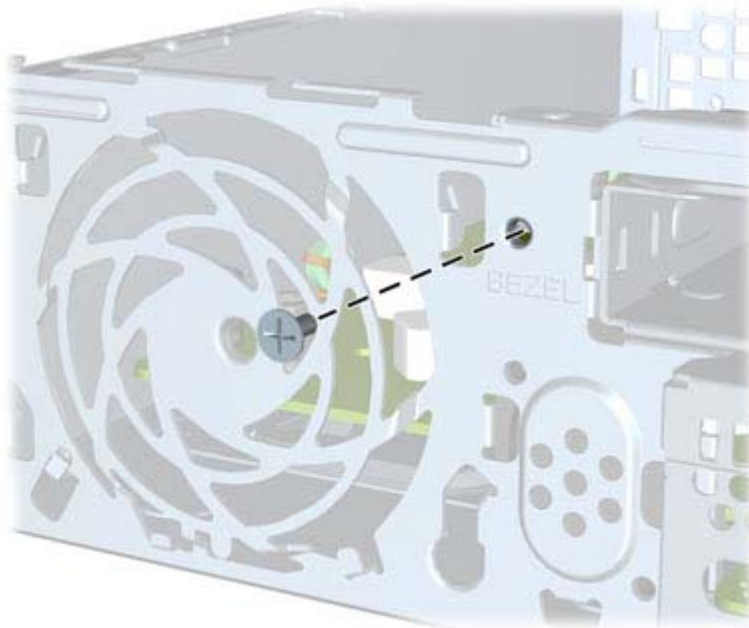
Figure 9-3 Retrieving the Front Bezel Security Screw
