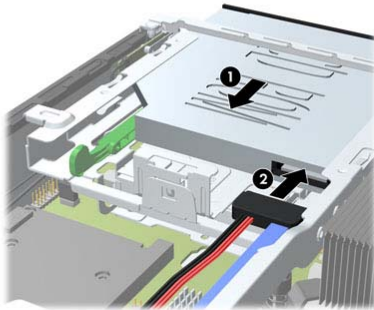
Figure 9-13 Installing the optical drive
