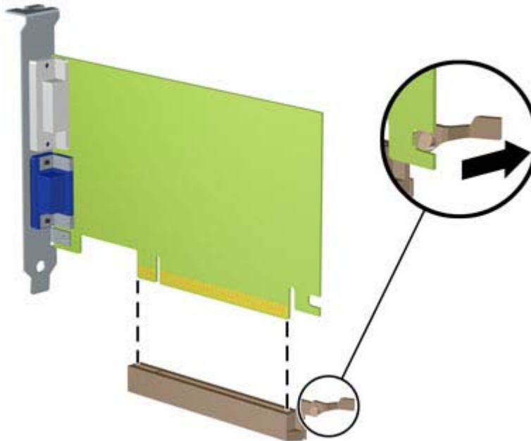
Figure 6-11 Removing a PCI Express x16 Expansion Card
