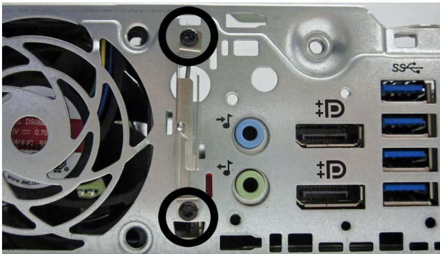
Figure 9-42 Removing the rear antenna – outside
