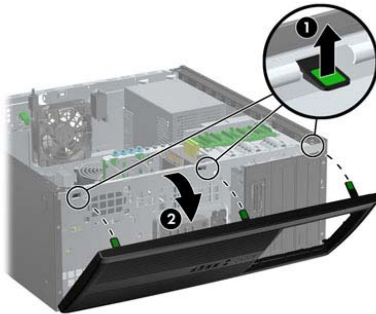
Figure 6-2 Removing the Front Bezel
