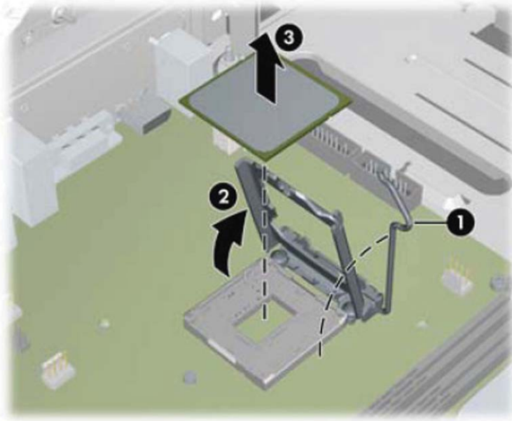
Figure 6-36 Removing the processor
