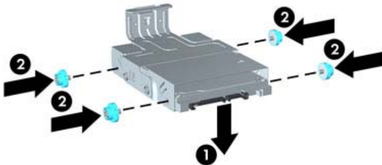
Figure 9-19 Lowering the hard drive and replacing the guide screws
