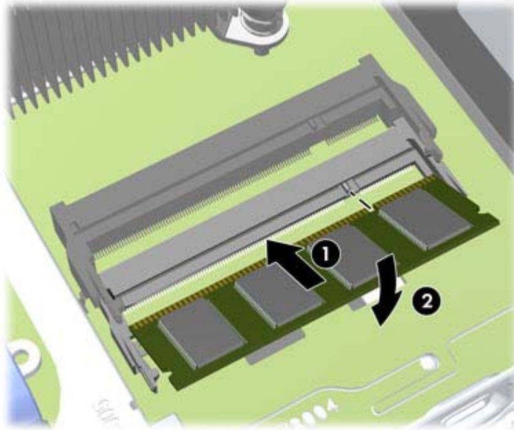
Figure 9-9 Installing a SODIMM
