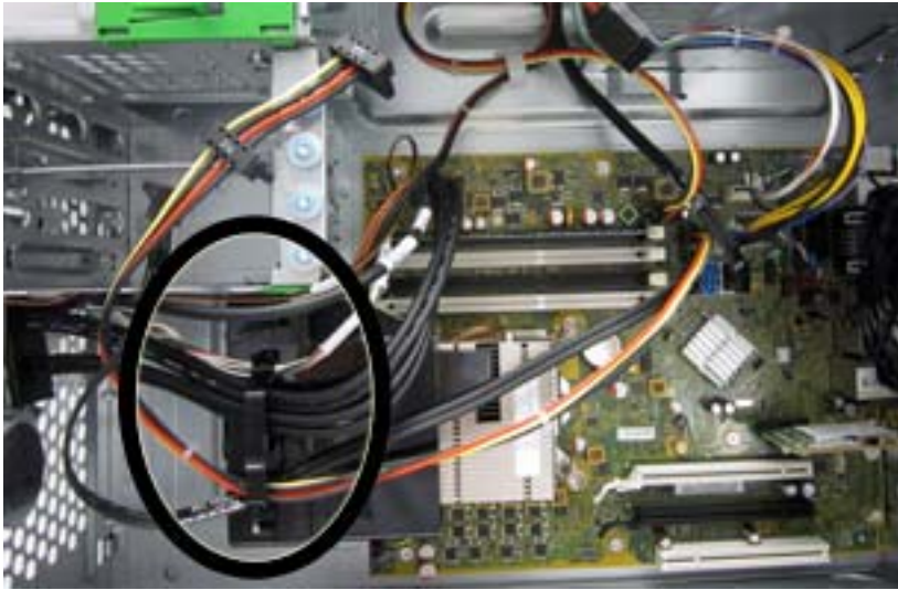
Figure 7-25 Removing the cables from atop the front fan assembly
