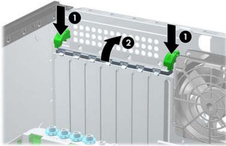
Figure 6-8 Opening the Expansion Slot Retainer
