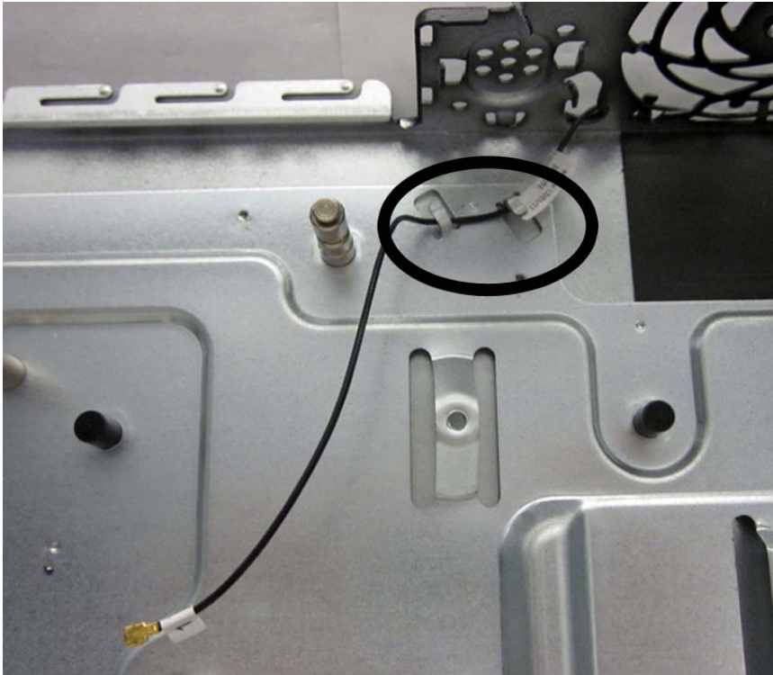
Figure 9-39 Removing the front antenna – inside
