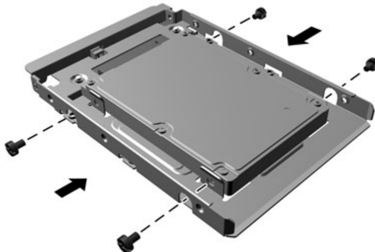
Figure 6-24 Securing the Drive in the Adapter Bracket
