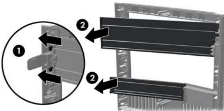
Figure 7-5 Removing a Bezel Blank
