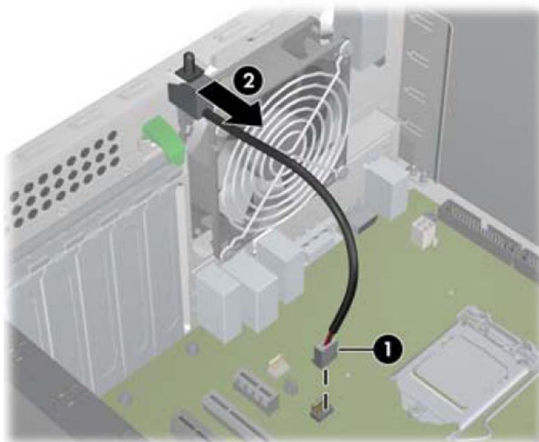
Figure 6-29 Removing the hood sensor
