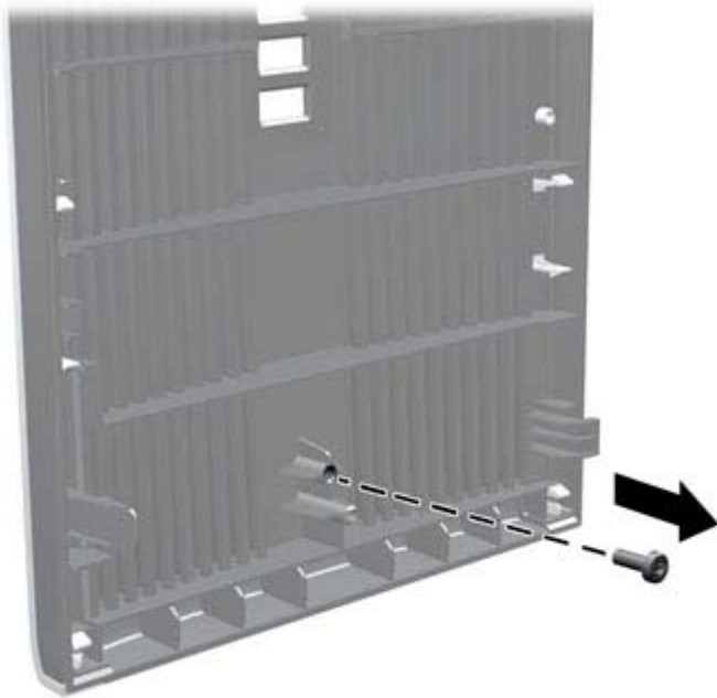
Figure 7-3 Retrieving the Front Bezel Security Screw
