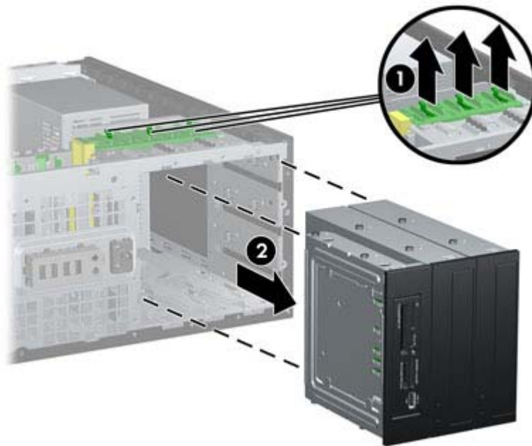
Figure 6-40 Releasing the 5.25-inch Drives from the Drive Bays (Minitower)
