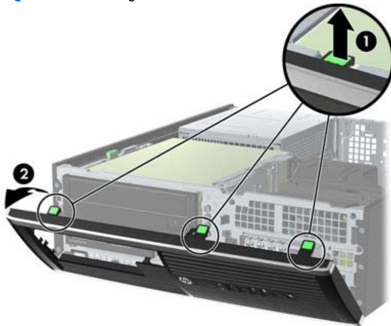
Figure 8-2 Removing the front bezel
