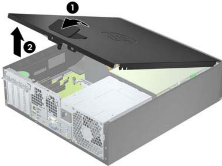
Figure 8-1 Removing the access panel
