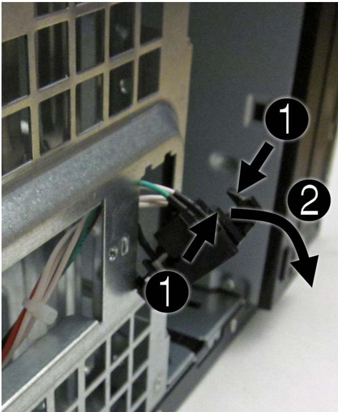
Figure 6-31 Removing the power switch assembly
