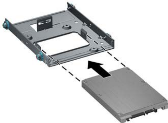
Figure 7-23 Installing the Drive in the Adapter Bracket
