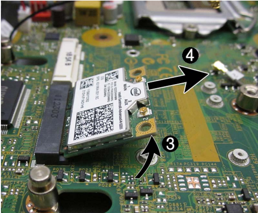
Figure 9-30 Removing the WLAN module
