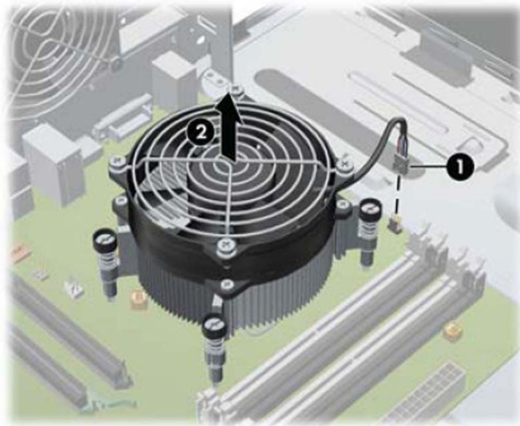
Figure 6-35 Removing the fan sink
