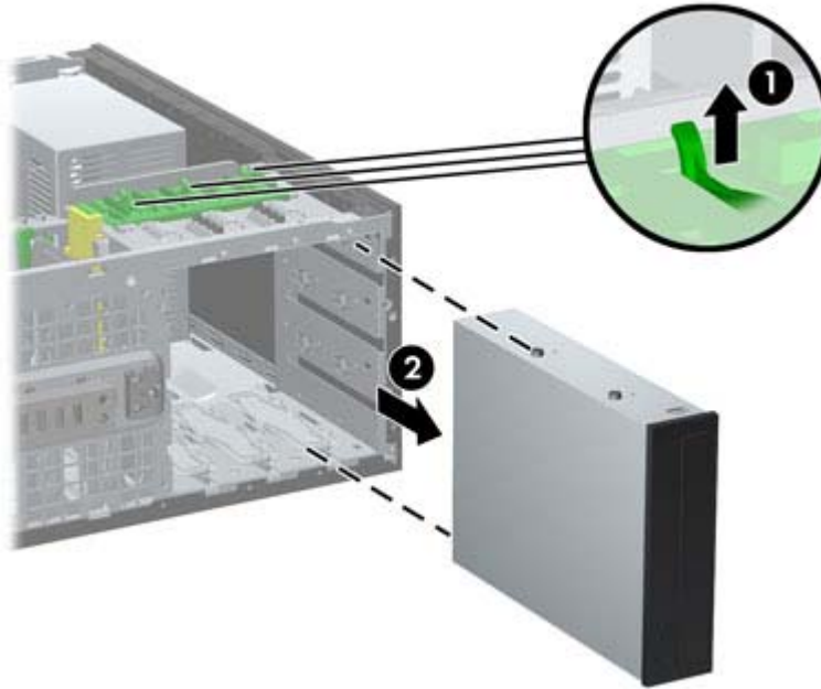
Figure 6-16 Removing a 5.25-inch Drive in the Minitower Configuration (Optical Drive shown)
