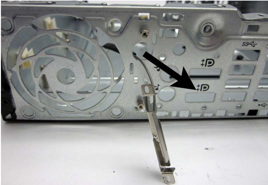
Figure 9-43 Removing the rear antenna
