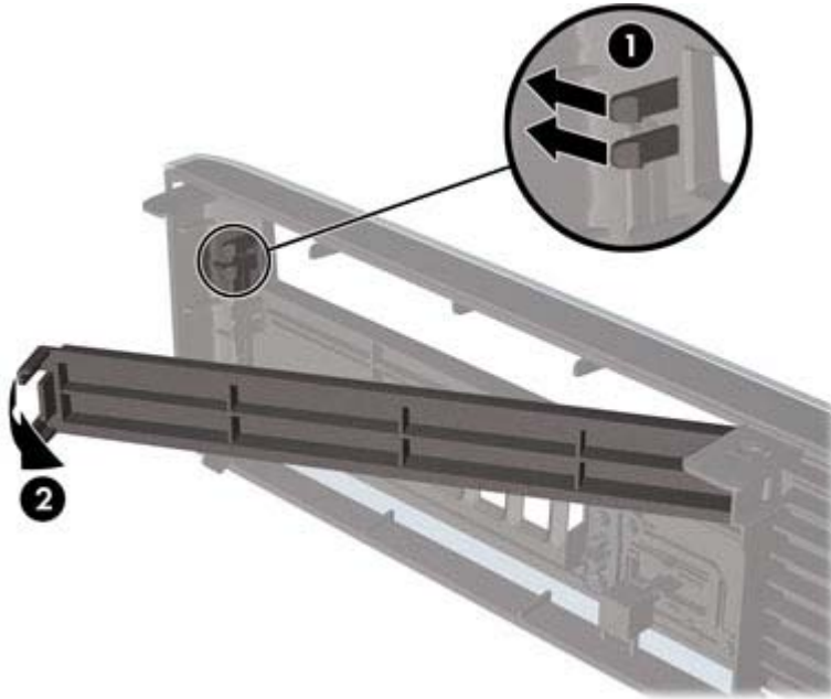
Figure 9-5 Removing a bezel blank
