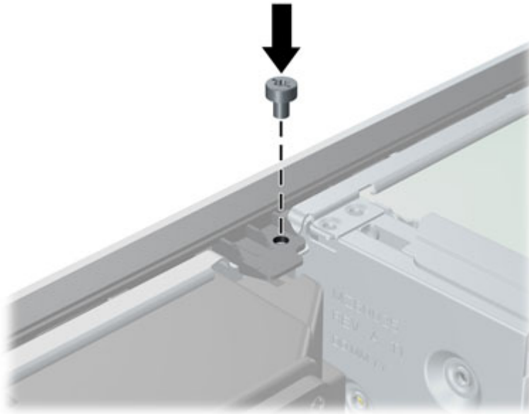
Figure 8-4 Installing the Front Bezel Security Screw
