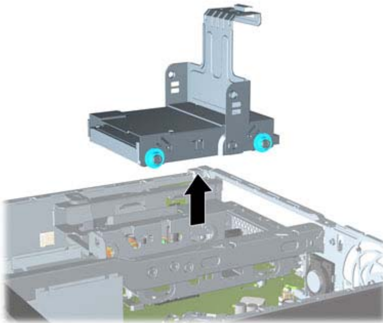
Figure 9-15 Removing the hard drive carrier
