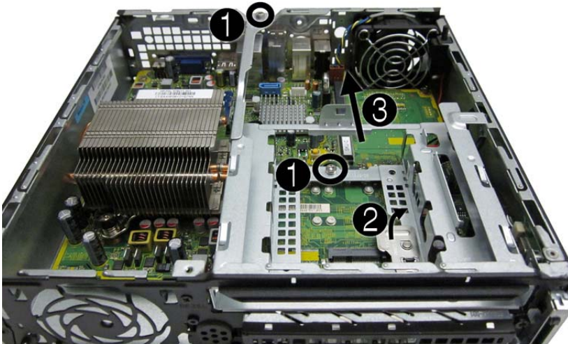
Figure 9-21 Removing the optical drive rail
