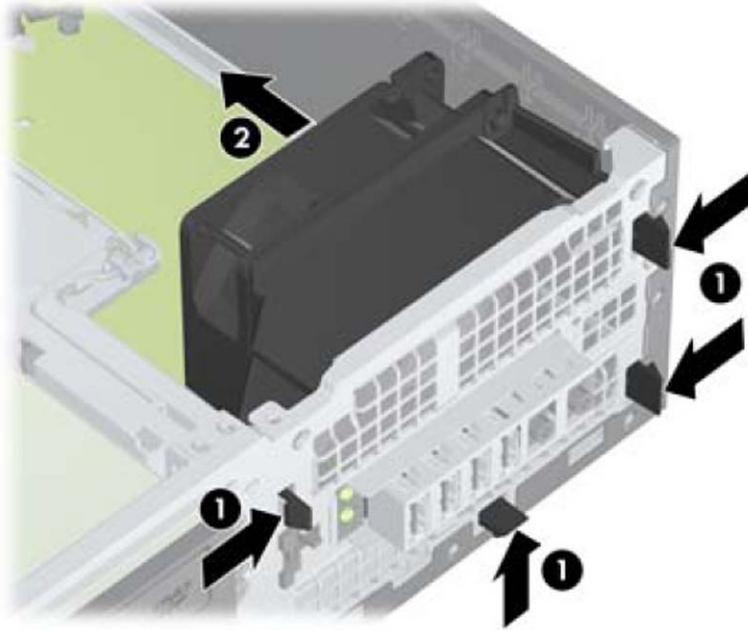
Figure 8-30 Removing the front fan
