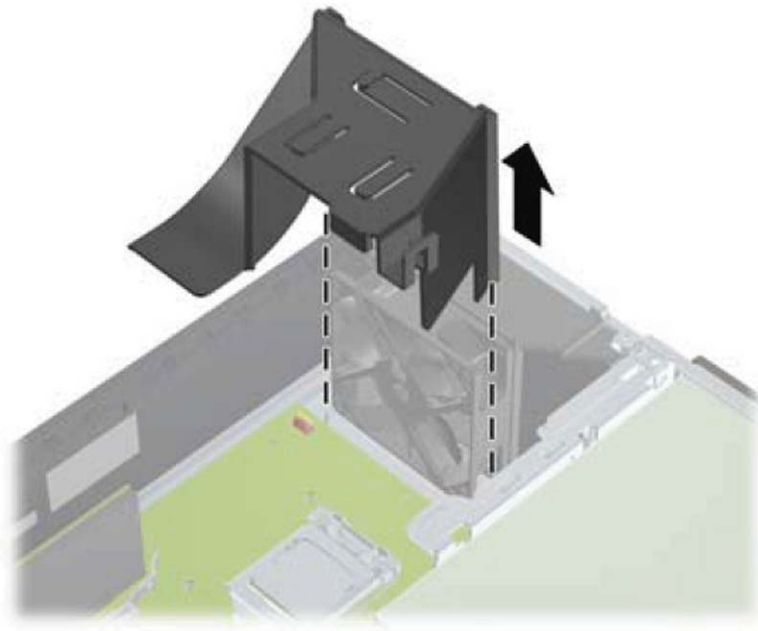
Figure 8-28 Removing the fan duct
