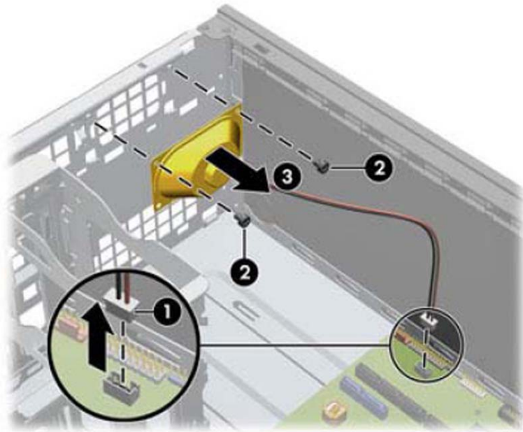
Figure 6-32 Removing the speaker
