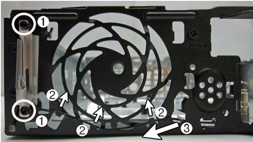
Figure 9-40 Removing the front antenna – outside
