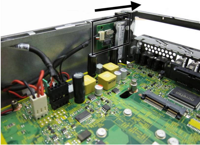
Figure 9-23 Removing the card reader
