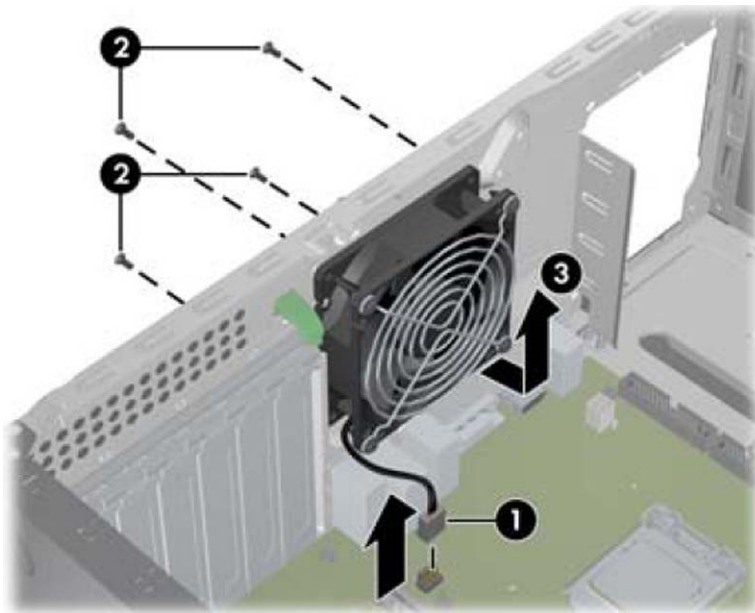
Figure 6-33 Removing the rear chassis fan
