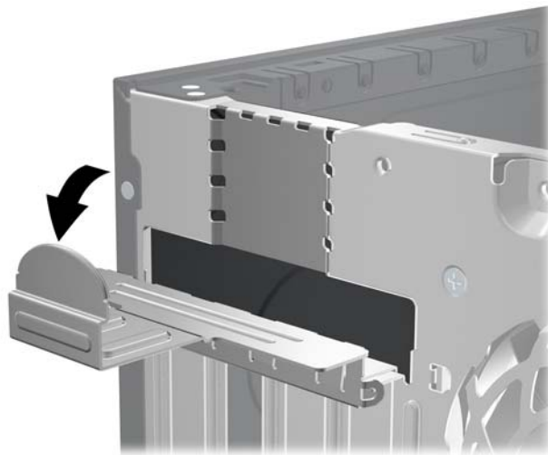
Figure 7-7 Opening the Expansion Slot Retainer
