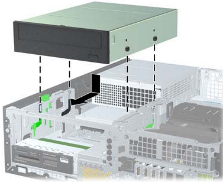
Figure 8-18 Installing the Optical Drive
