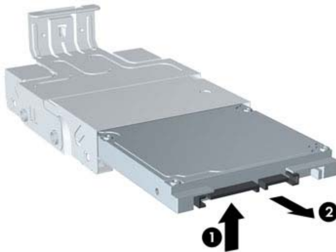
Figure 9-17 Removing the hard drive from the carrier
