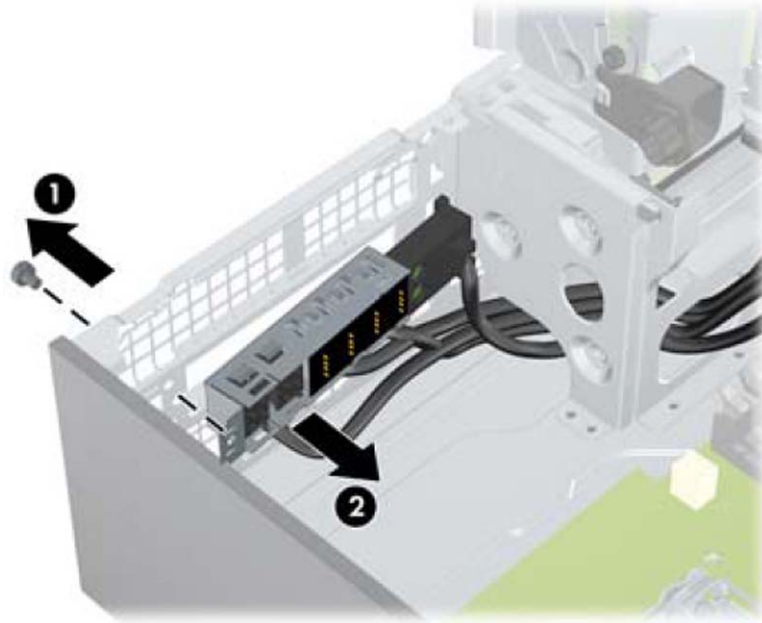
Figure 8-33 Removing the front I/O, power switch/LED assembly screw
