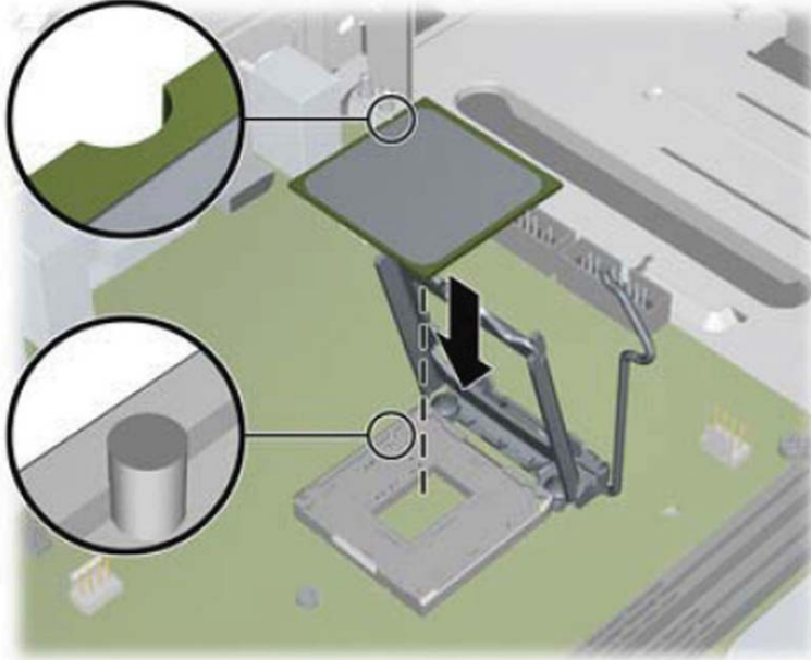
Figure 6-37 Installing the processor
