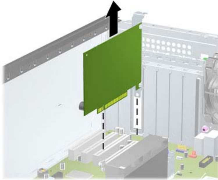
Figure 6-10 Removing a Standard PCI Expansion Card
