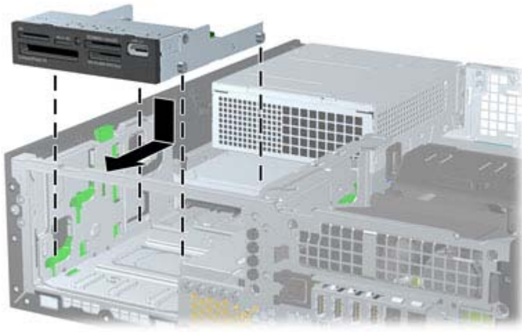
Figure 8-22 Installing a Drive into the 3.5-inch Drive Bay (Media Card Reader Shown)
