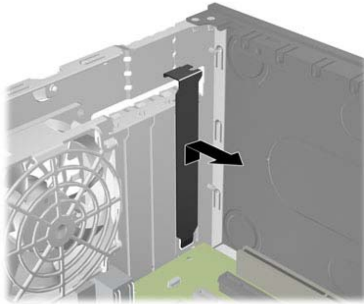
Figure 7-8 Removing an Expansion Slot Cover
