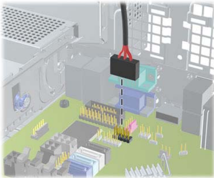
Figure 8-19 Disconnecting the Media Card Reader USB Cable
