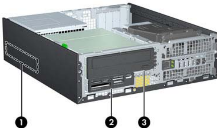
Figure 8-14 Drive Positions
