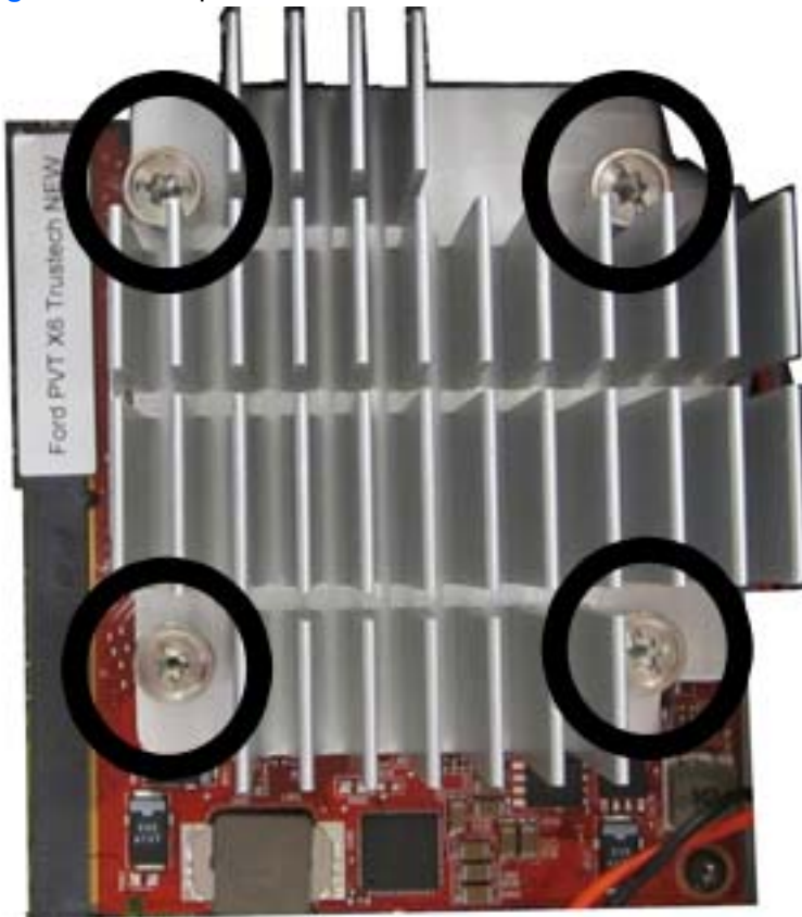
Figure 9-33 Graphics board heat sink screws
