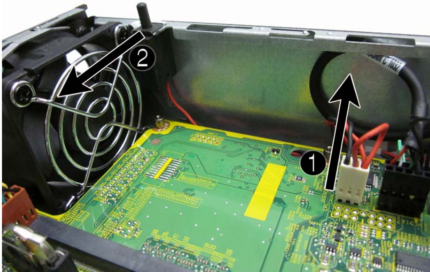
Figure 9-31 Removing the hood sensor
