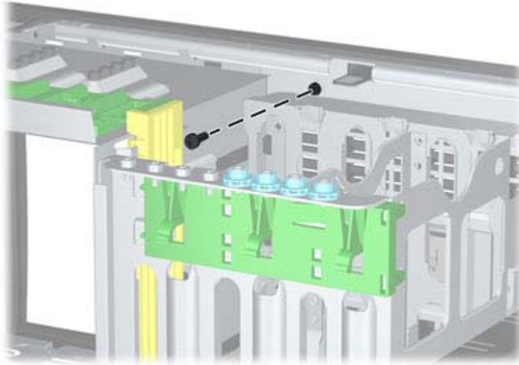
Figure 6-4 Installing the Front Bezel Security Screw
