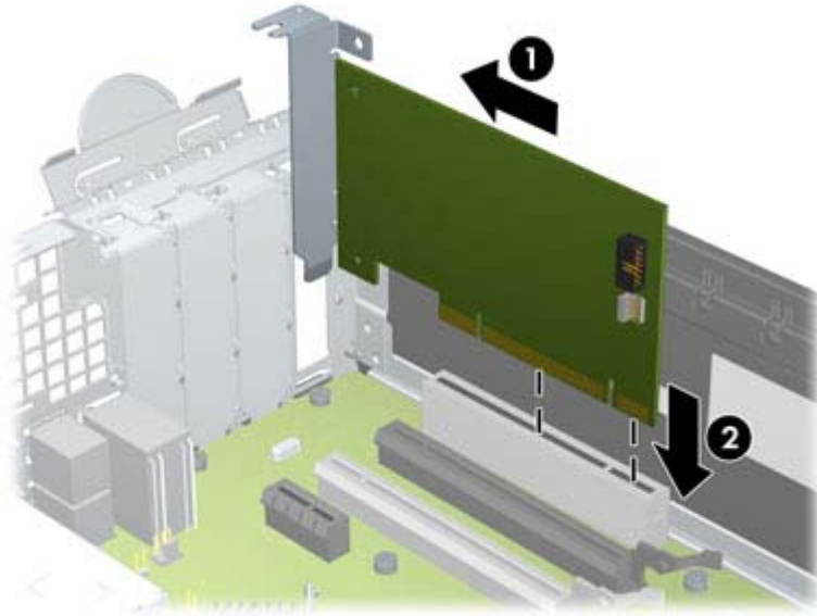
Figure 8-11 Installing an Expansion Card
