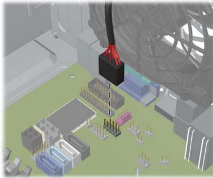
Figure 7-20 Connecting the Media Card Reader USB Cable
