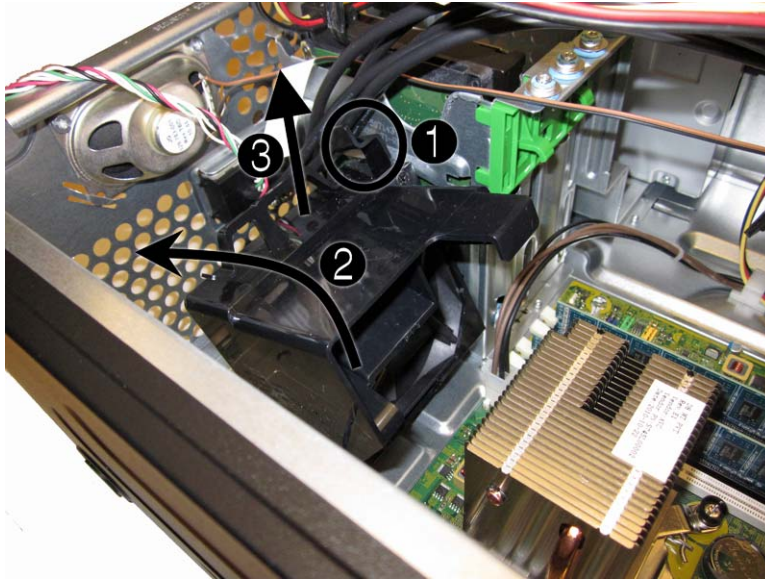
Figure 7-26 Removing the front fan assembly
