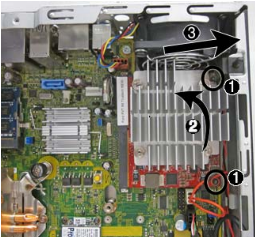
Figure 9-32 Removing the graphics board
