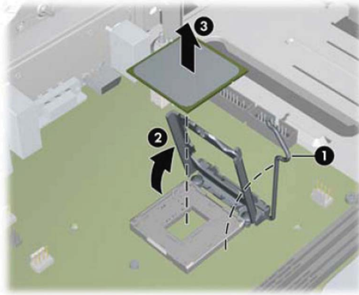
Figure 9-27 Removing the processor
