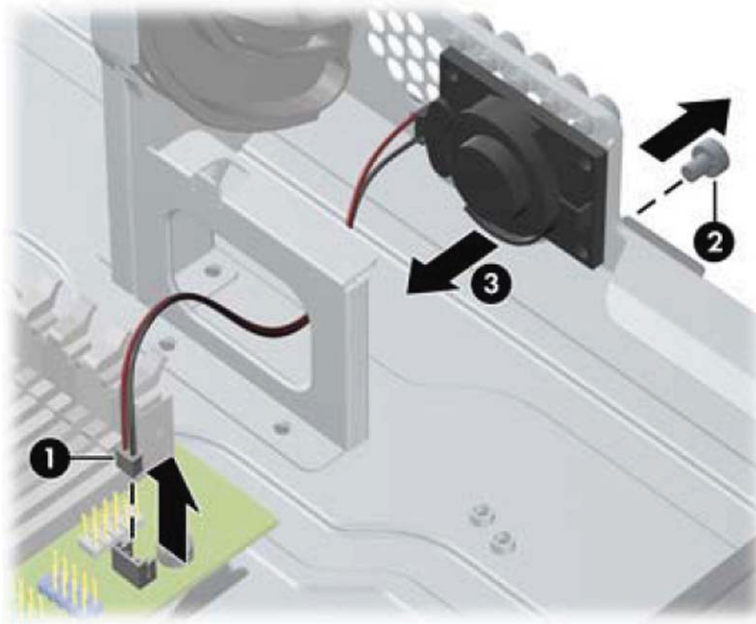
Figure 8-34 Removing the speaker
