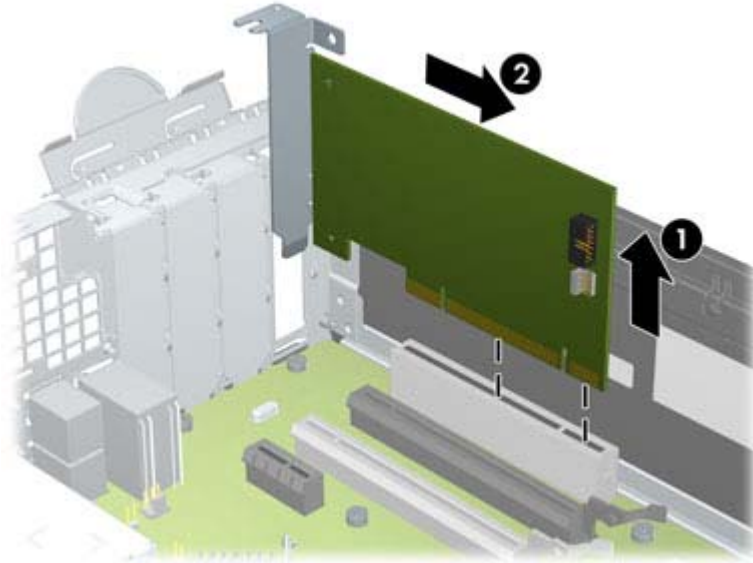
Figure 8-9 Removing a Standard PCI Expansion Card
