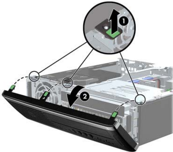
Figure 9-2 Removing the front bezel
