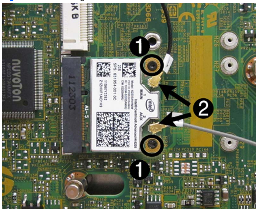
Figure 9-29 Removing the WLAN module
