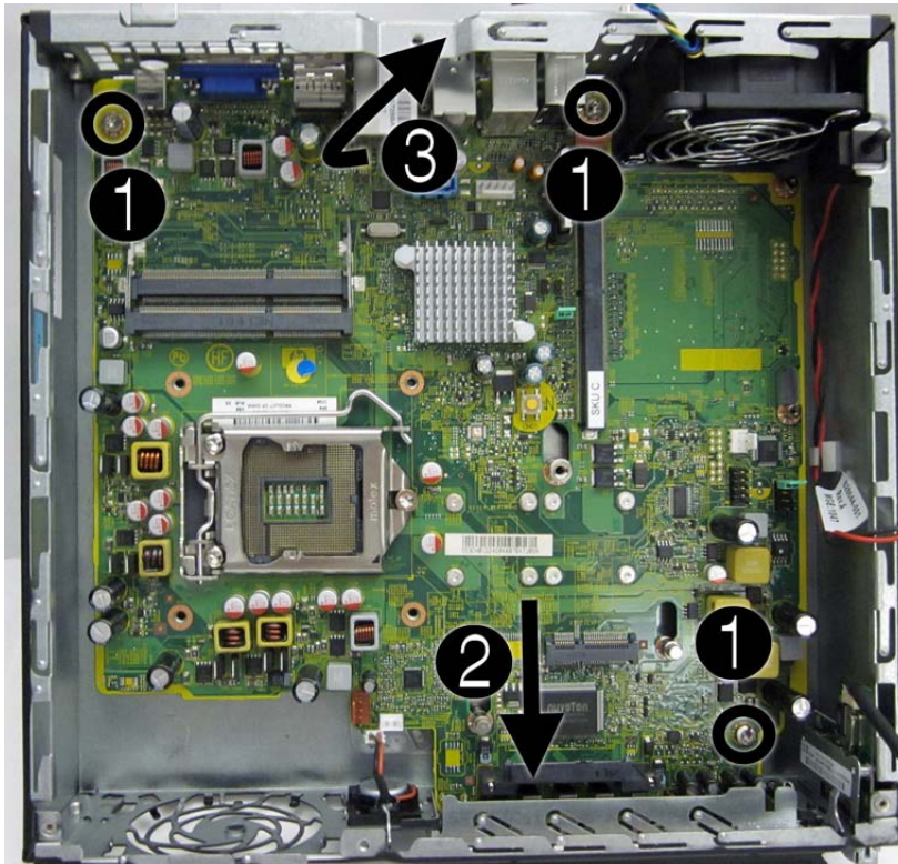
Figure 9-36 Removing the system board
