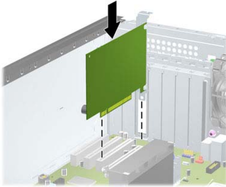
Figure 6-12 Installing an Expansion Card
