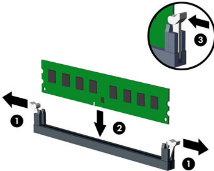
Figure 8-6 Installing a DIMM
