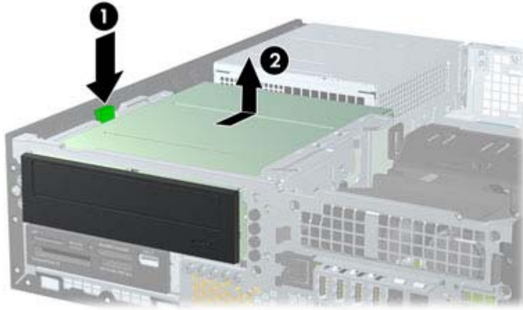
Figure 8-16 Removing the 5.25-inch Drive
