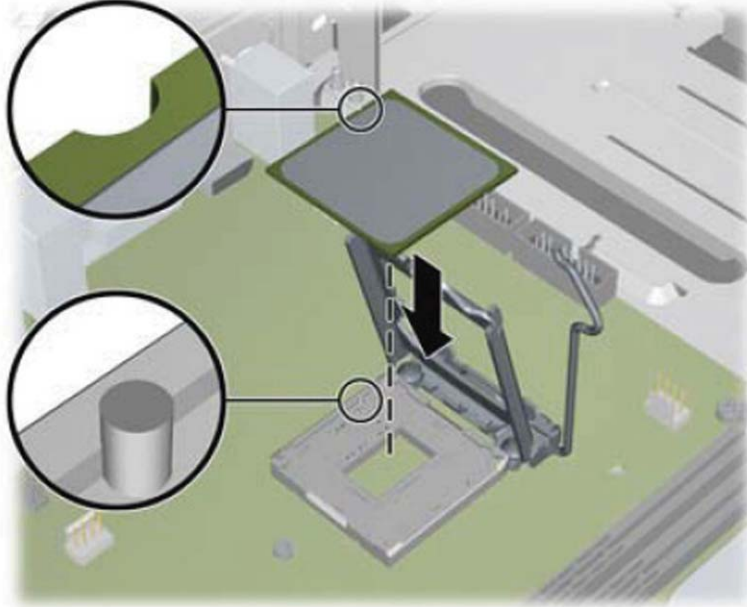
Figure 9-28 Replacing the processor
