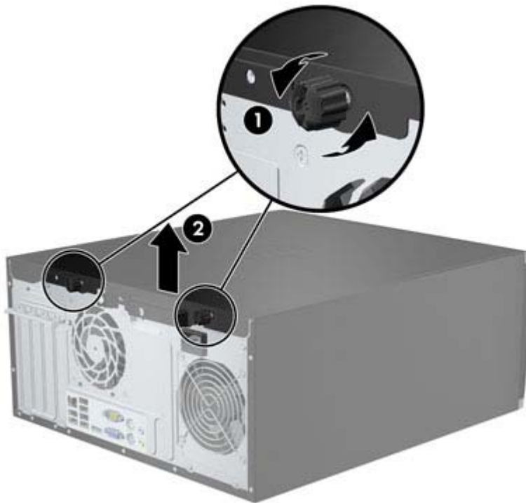
Figure 7-1 Removing the Computer Access Panel
