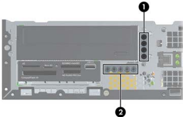
Figure 8-15 Extra Guide Screw Locations
