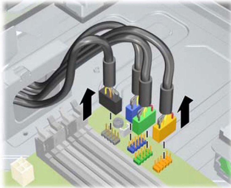
Figure 8-32 Disconnecting the front I/O, power switch/LED assembly cables
