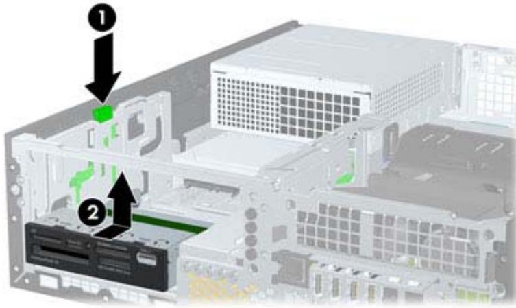
Figure 8-20 Removing a 3.5-inch Drive (Media Card Reader Shown)
