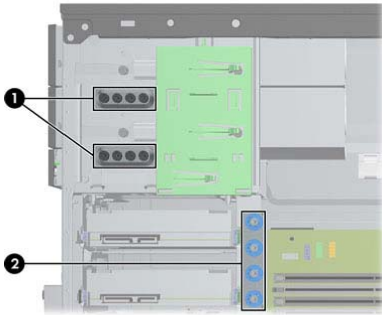
Figure 7-14 Extra Guide Screw Locations
