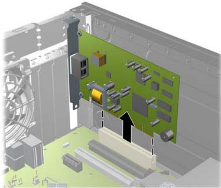
Figure 7-9 Removing a Standard PCI Expansion Card
