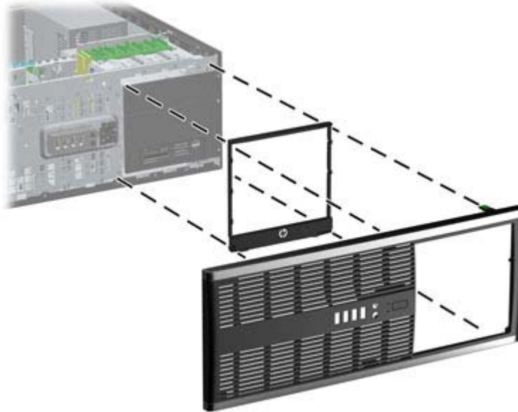
Figure 6-42 Changing from a Minitower to a Desktop Configuration
