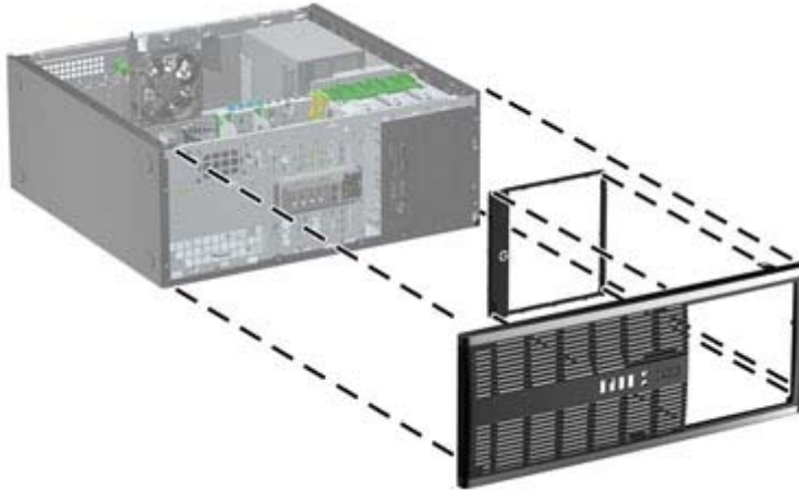
Figure 6-45 Changing from a Desktop to a Minitower Configuration
