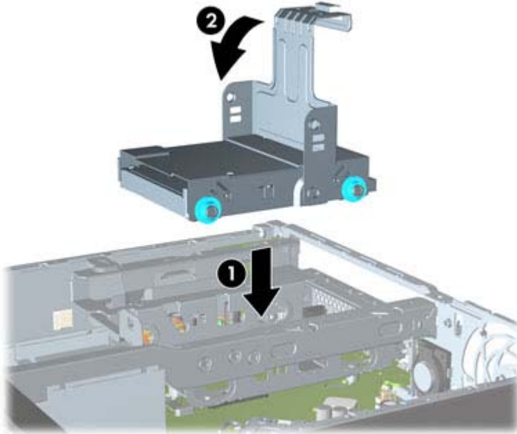
Figure 9-20 Installing the hard drive carrier
