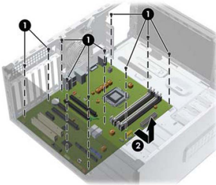
Figure 6-39 Removing the system board
