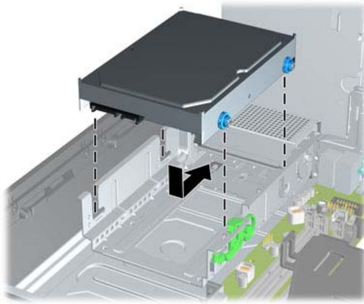
Figure 8-27 Installing the Hard Drive
