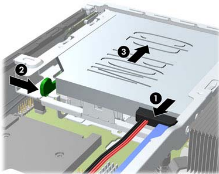
Figure 9-11 Removing the optical drive
