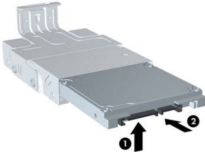
Figure 9-18 Sliding the hard drive into the carrier
