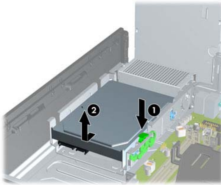
Figure 8-25 Removing the Hard Drive
