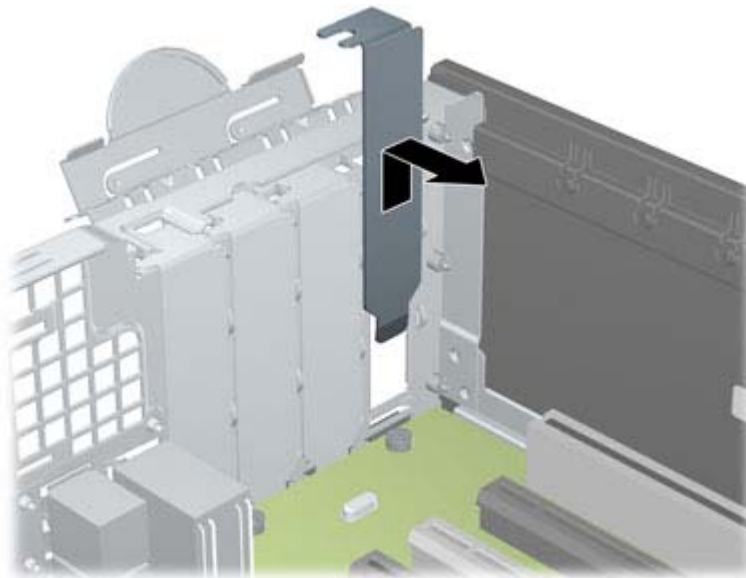
Figure 8-8 Removing an Expansion Slot Cover
