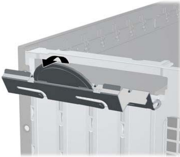
Figure 8-7 Opening the Expansion Slot Retainer
