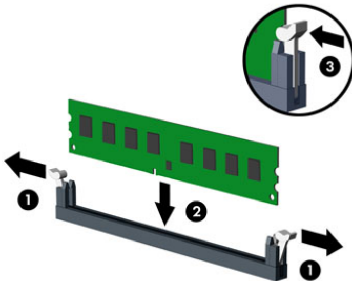
Figure 6-7 Installing a DIMM
