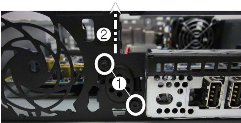
Figure 9-24 Removing the speaker
