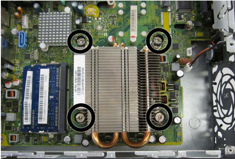
Figure 9-25 Loosening the heat sink screws
