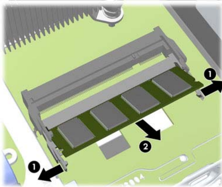
Figure 9-8 Removing a SODIMM
