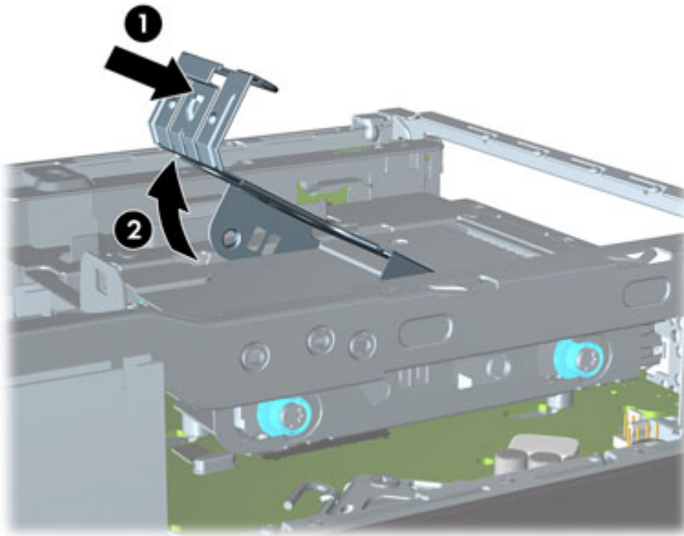
Figure 9-14 Unlocking the hard drive carrier
