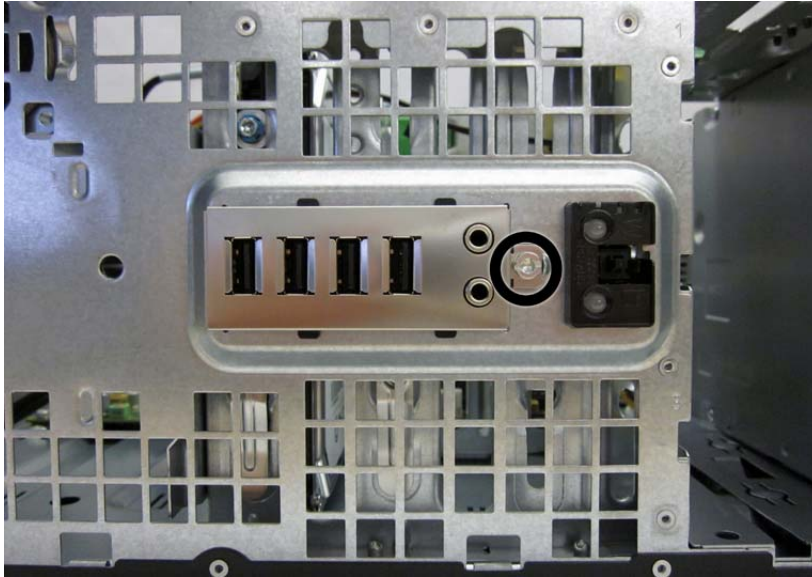
Figure 6-30 Removing the front I/O, USB, power switch assembly
