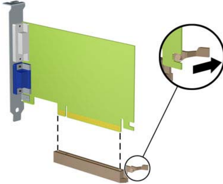
Figure 7-10 Removing a PCI Express x16 Expansion Card
