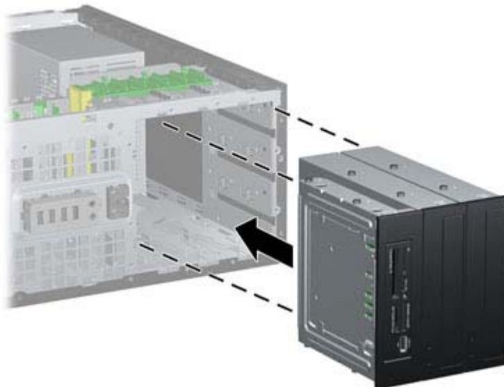
Figure 6-44 Installing a Drive in the Minitower Configuration
