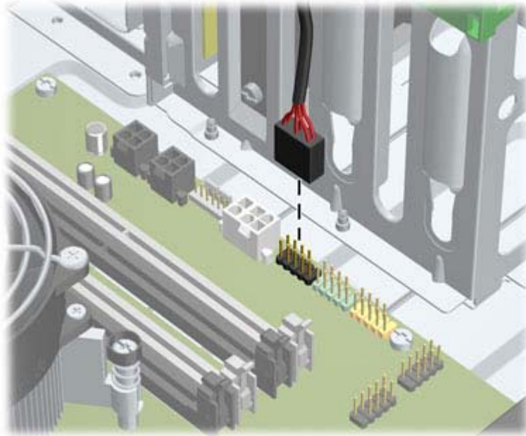
Figure 6-14 Disconnecting the Media Card Reader USB Cable
