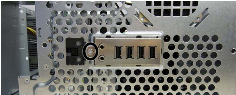
Figure 7-27 Removing the front I/O assembly screw
