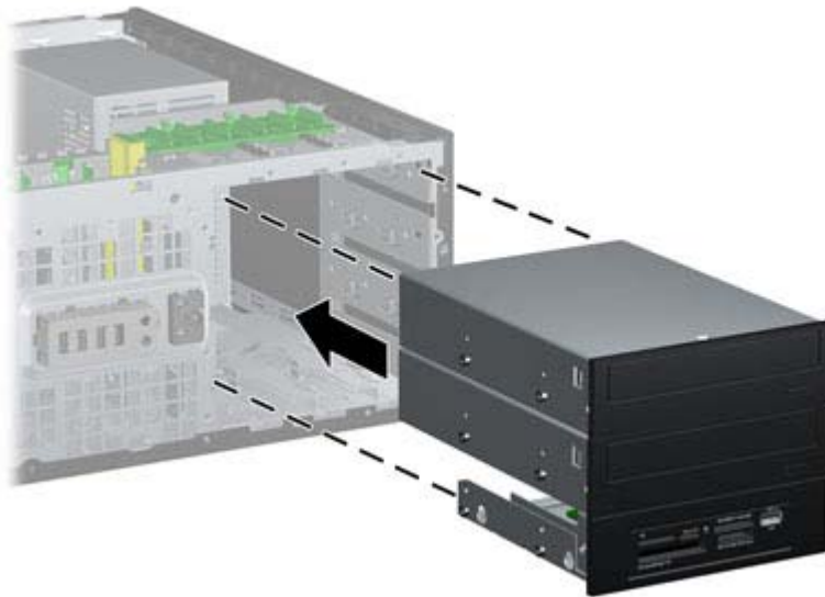
Figure 6-41 Installing a Drive in the Desktop Configuration
