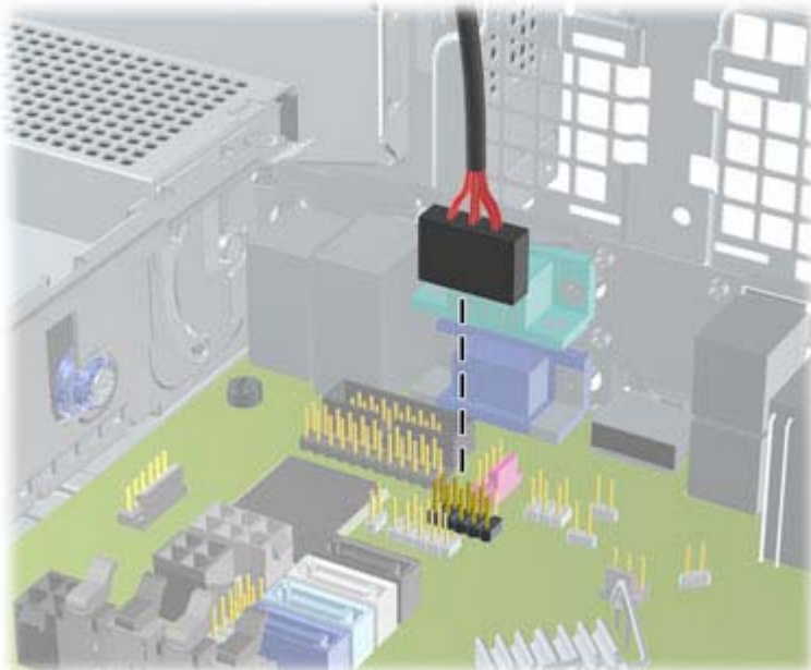
Figure 8-23 Connecting the Media Card Reader USB Cable
