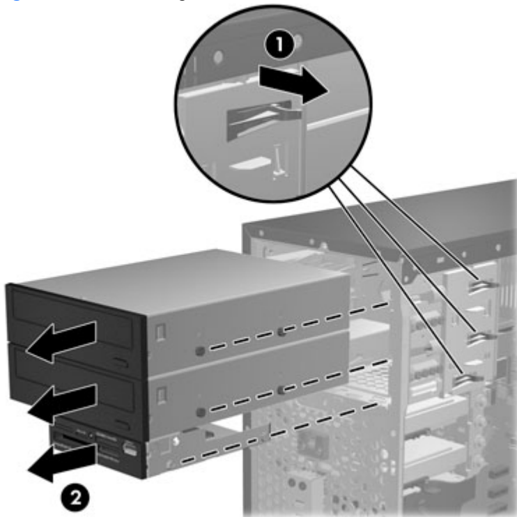
Figure 7-17 Removing the Drives
