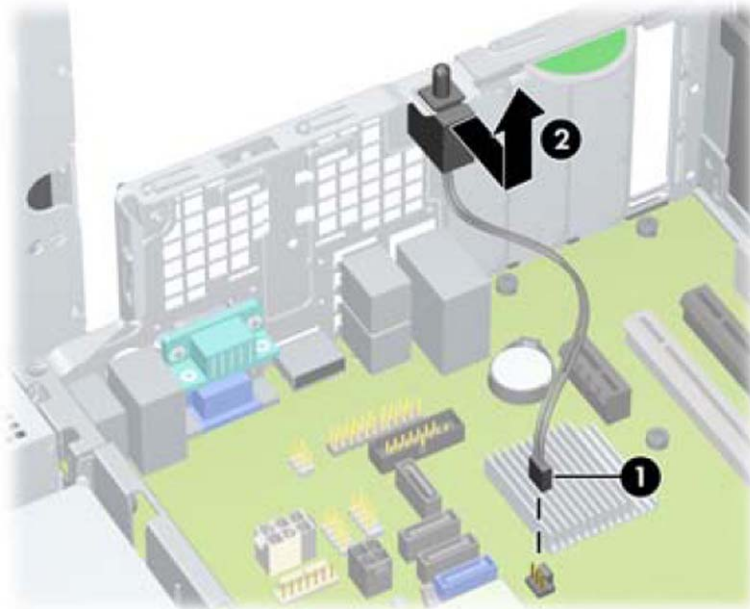
Figure 8-31 Removing the hood sensor from the chassis fan
