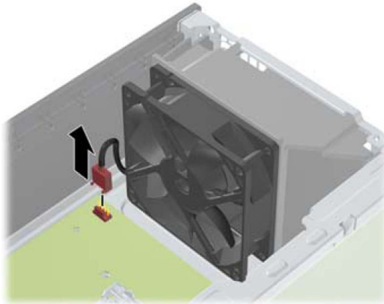
Figure 8-29 Disconnecting the front fan cable
