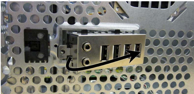
Figure 7-28 Removing the front I/O assembly
