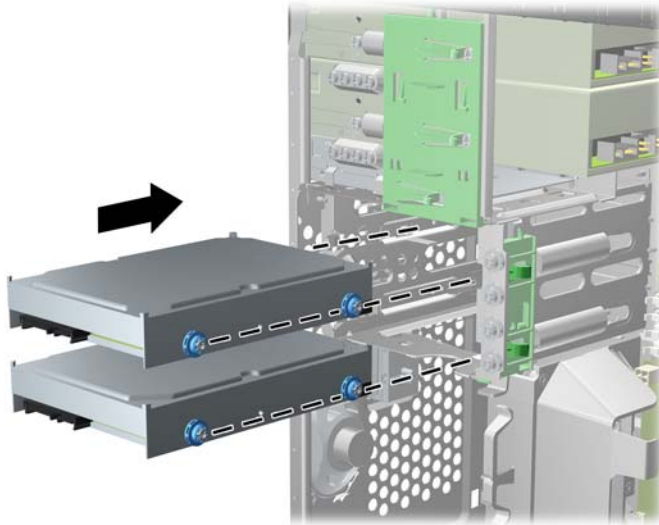
Figure 7-24 Sliding a Hard Drive into the Drive Bay
