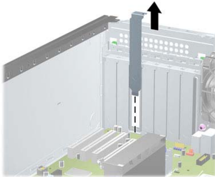
Figure 6-9 Removing an Expansion Slot Cover
