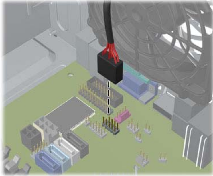
Figure 7-16 Disconnecting the Media Card Reader USB Cable
