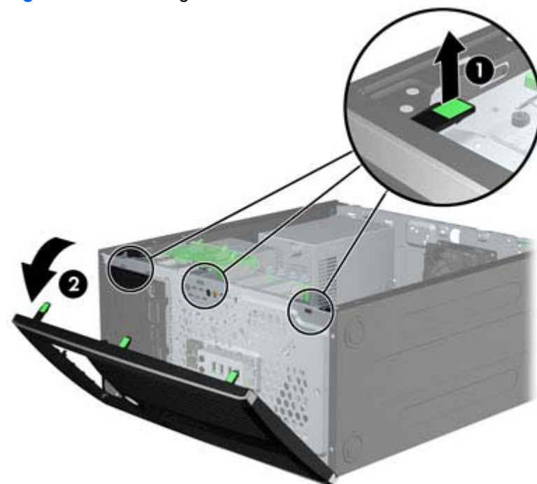
Figure 7-2 Removing the Front Bezel
