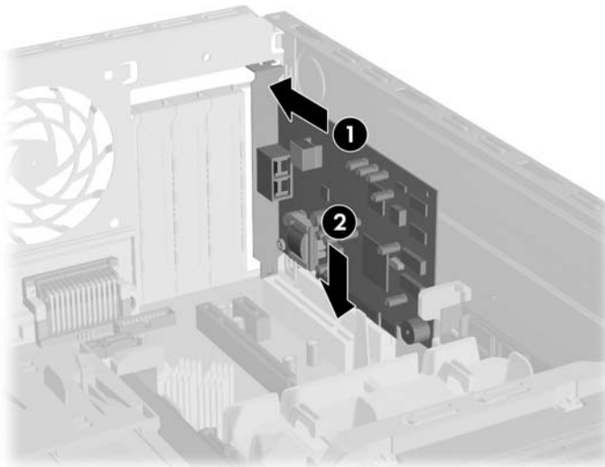
Figure 2-12 Installing an Expansion Card
