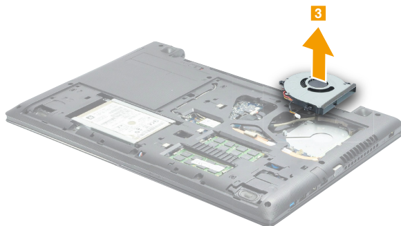
Figure 7. Removal steps of fan assembly (continued)
