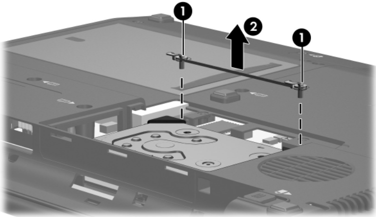
Removing the Hard Drive Bracket
