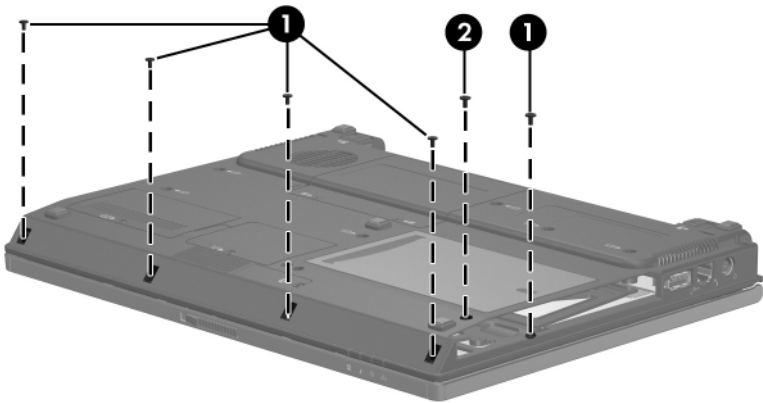
Torx8 T8M2.5×4.0 Screw Locations
