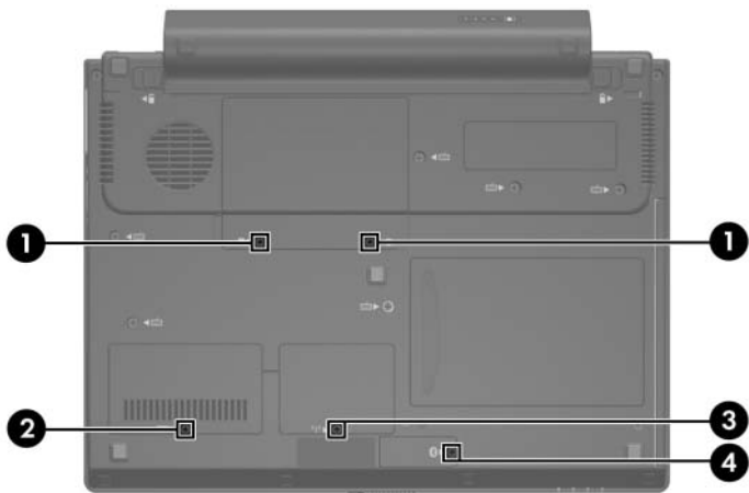
Phillips PM2.0x5.0 Screw Locations
