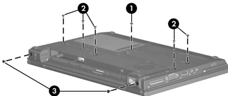
Torx8 T8M2.5×7.0 Screw Locations
