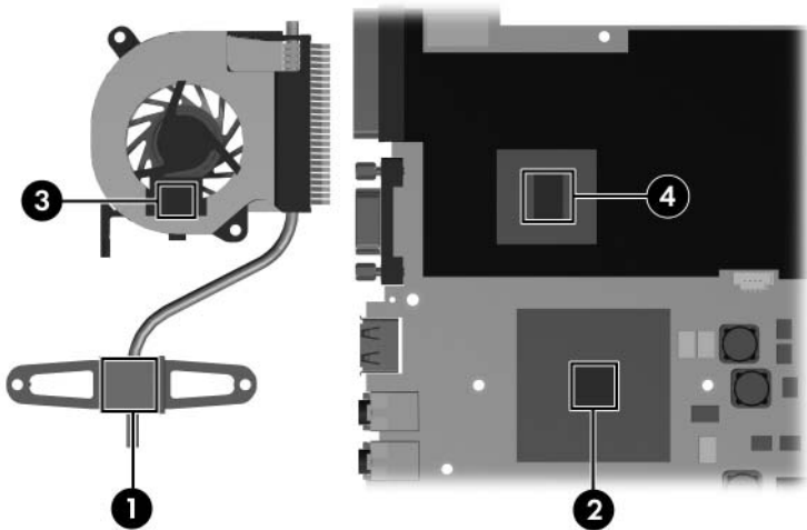
Thermal Paste and Thermal Pad Locations
