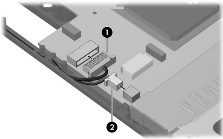
Disconnecting the LED Board Cable and the Speaker Cable
