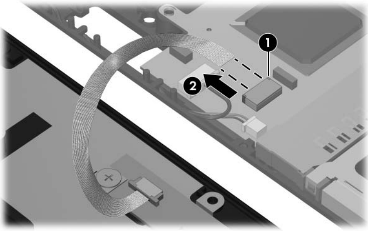
Disconnecting the Fingerprint Reader Board Cable
