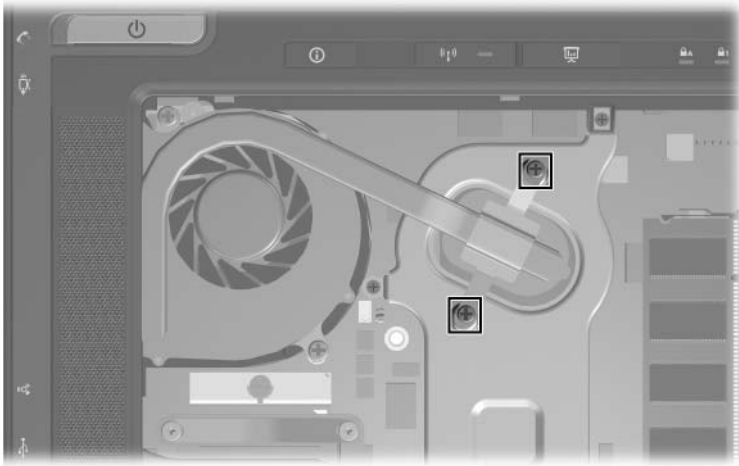
Phillips PM2.5×7.0 Captive Screw Locations
