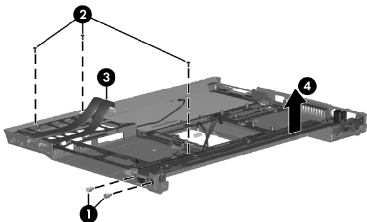
Remove the System Board Frame
