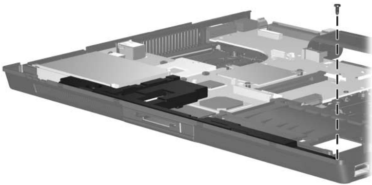
Torx8 T8M2.5×4.0 Screw Location
