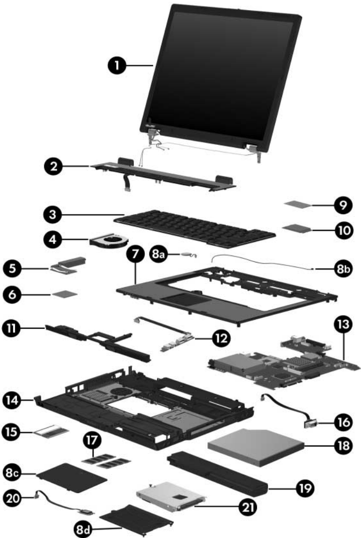
Computer Major Components
