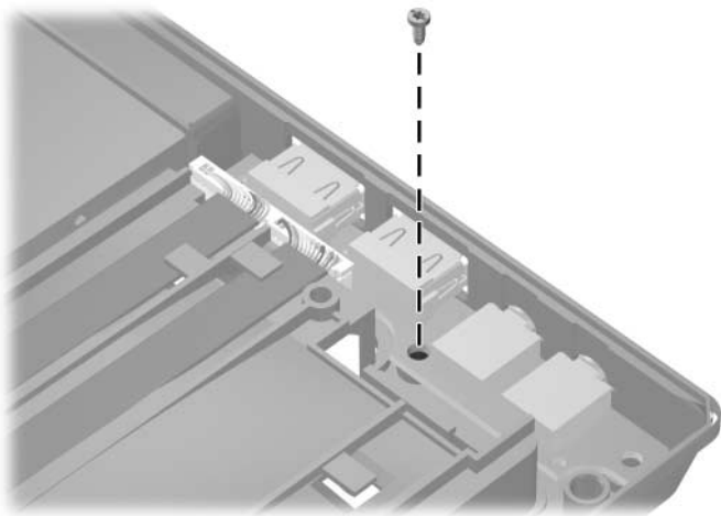
Phillips PM1.5×3.0 Screw Location
