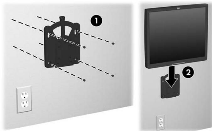
Figure 3-14 Mounting the Monitor to the Wall Using Quick Release
