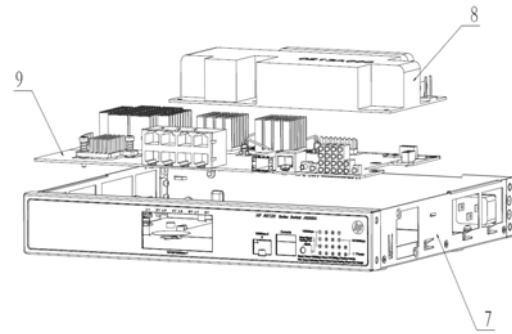
Figure 4 Remove the PCB and Power Module
