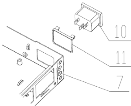
Figure 5 Remove the Cable connector
