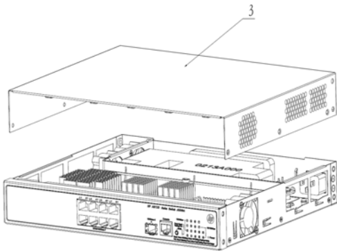
Figure 2 Remove Cover 3
