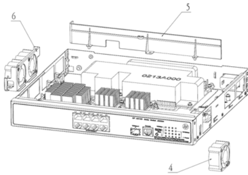
Figure 3 Remove the Fan and Part 5
