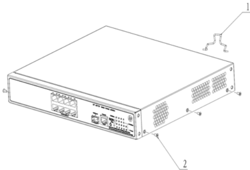
Figure 1 Unscrew the Power Cable Holder 1 and screw 2
