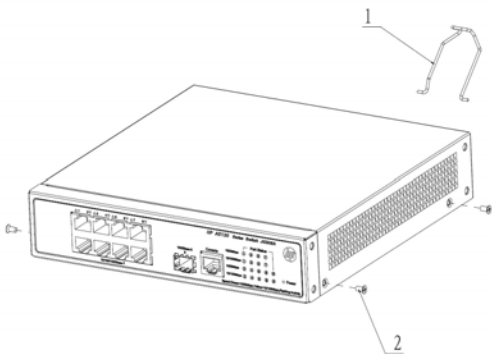
Figure 1 Remove mounting angle
