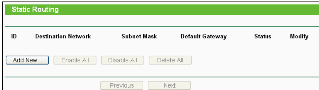
Figure 4-63 Static Routing
