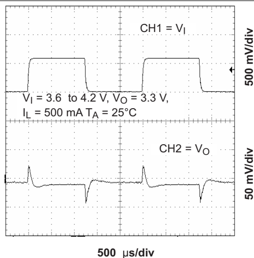
Figure 11. Line Transient Response (MAIN)
