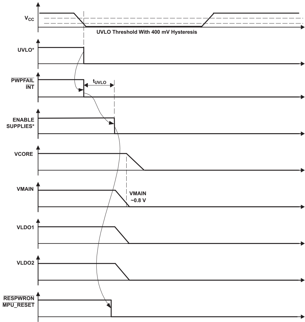
Figure 32. State2-State4 Transition
