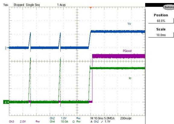
Figure 41: Recovery from Hiccup CH2:Vout, CH3:PGood, CH4:Iout
