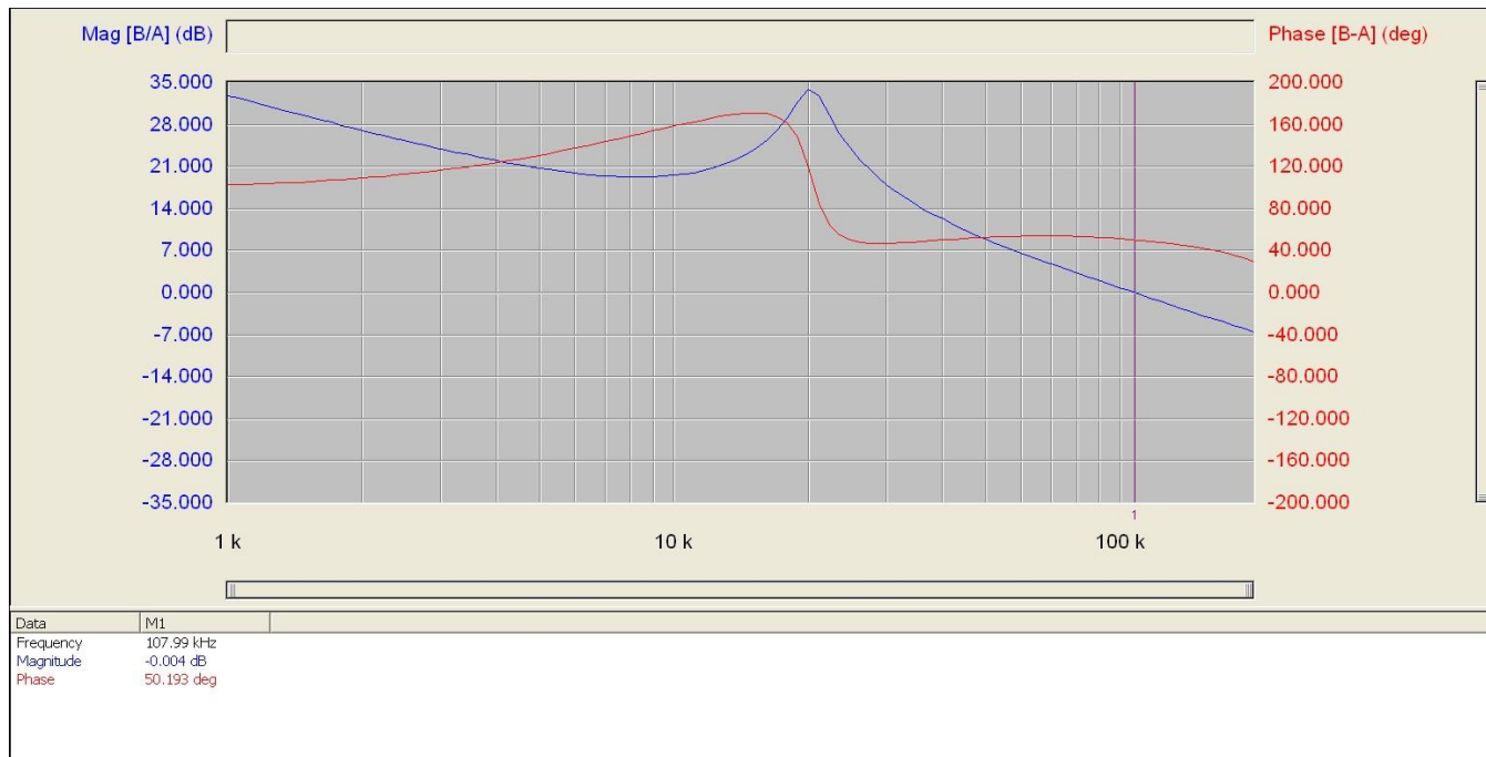
Figure 46: Bode Plot with 25A load: Fo = 108 kHz, Phase Margin = 50.2 Degrees
