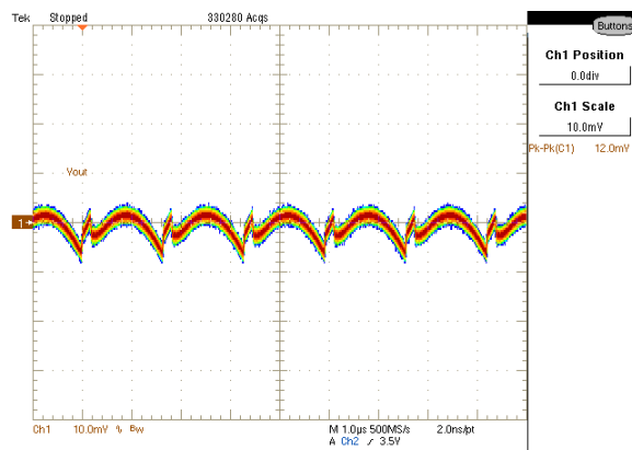
Figure 43: Output Voltage Ripple at full load CH1:Vout
