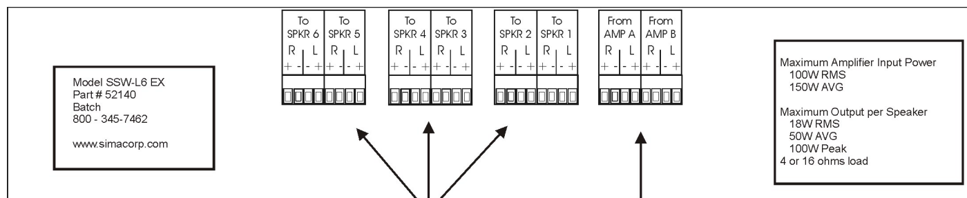
Figure 2, Rear Panel (SSW-L6 EX shown)
