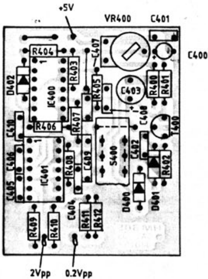
④ CAL.-BOARD
