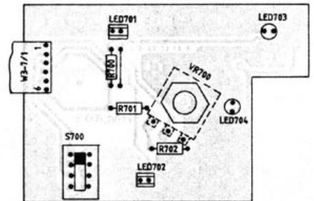
⑦ DELAY-BBOARD
