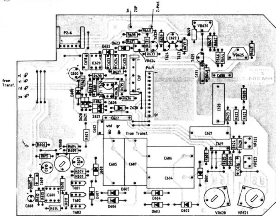
⑥ Z-BOARD
