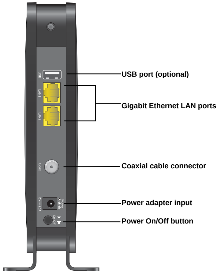
Figure 3. Modem router rear panel
