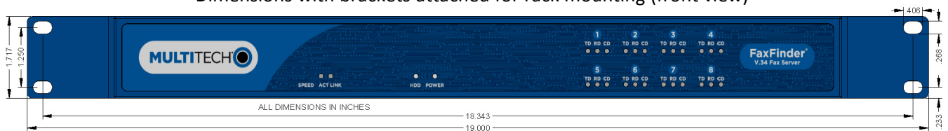
Dimensions with brackets attached for rack mounting (front view)
