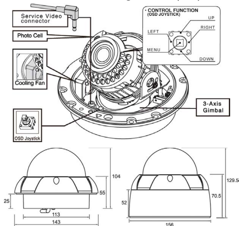
General Feature Diagram Unit: (mm)
