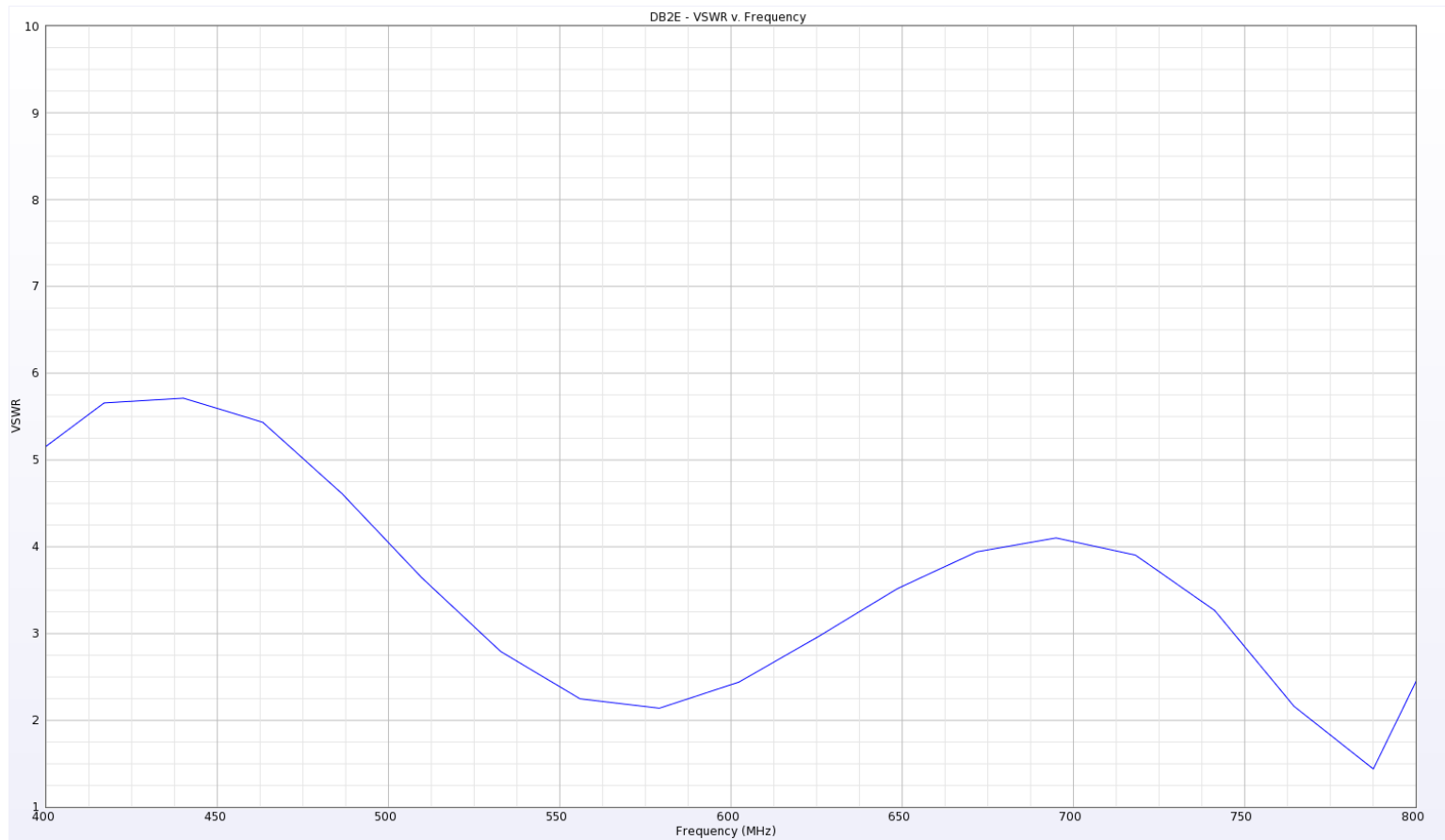
Illustration 5: DB2 - Computed VSWR versus Frequency. Balun included. 75 ohm reference. Measured better, see next plot.
