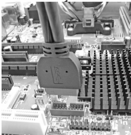
USB 3.0 20-Pin Adapter
