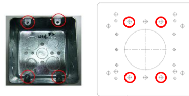
Image 42-2 Double gang box
