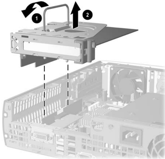
Removing the Expansion Card Assembly
