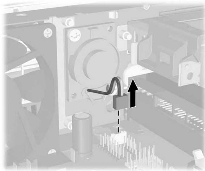
Disconnecting the Speaker Cable
