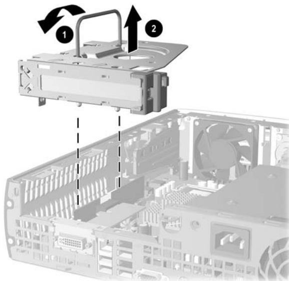
Removing the Expansion Card Assembly
