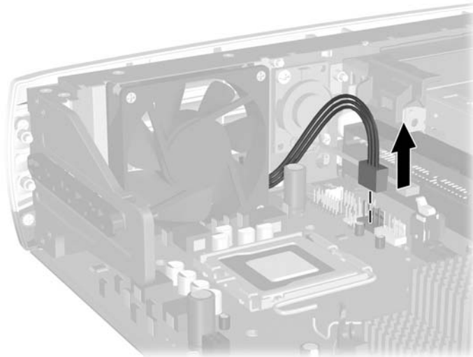
Disconnecting the Fan Cable
