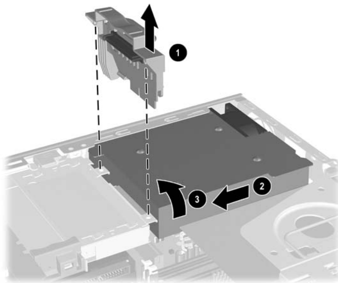
Removing the Power Supply
