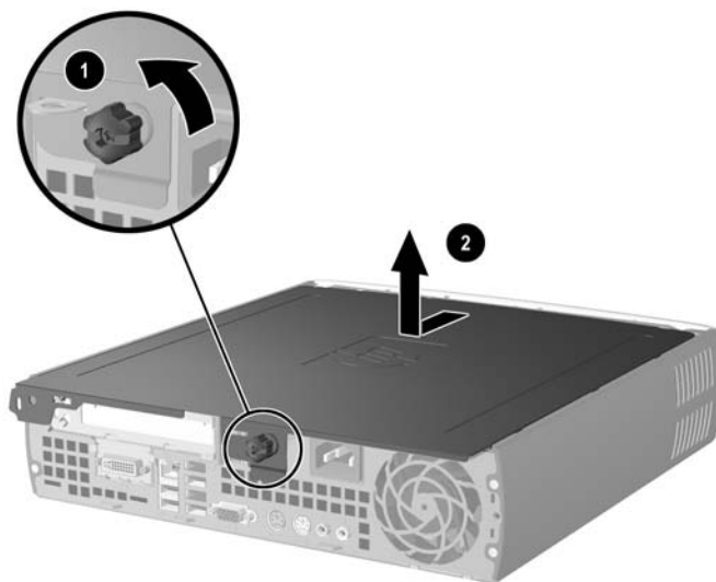
Removing the Access Panel
