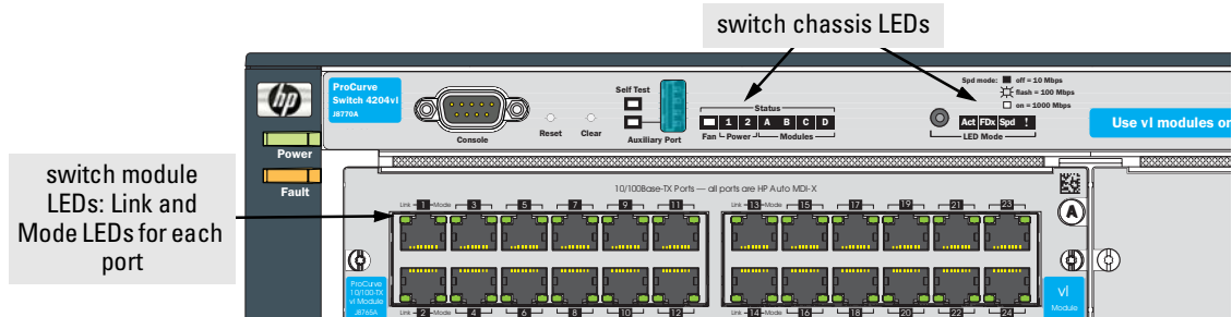
Figure 2-6. Switch LEDs
