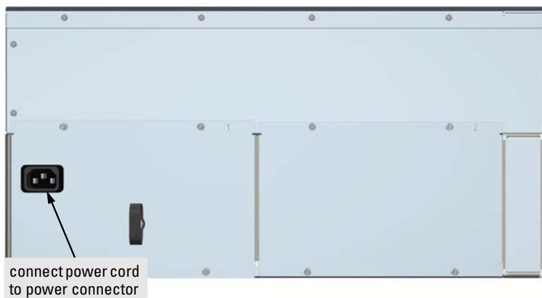
Figure 2-5. Connecting power to the Switch
