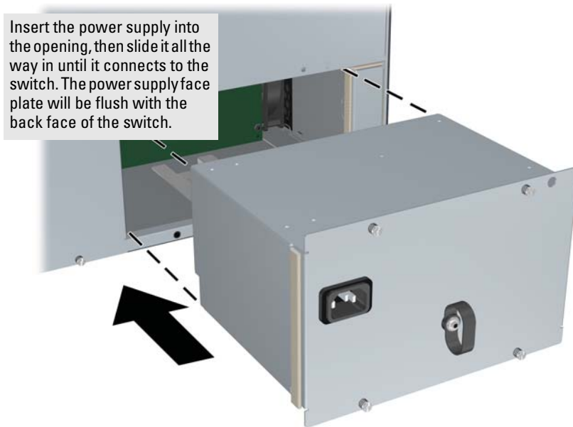
Figure 2-3. Installing a power supply
