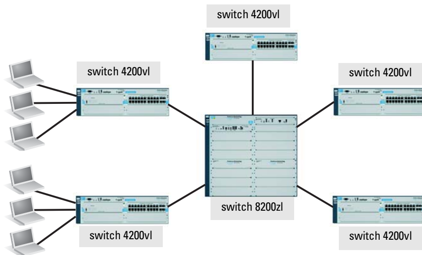
Figure 2-18. 10-GbE Aggregation Topology
