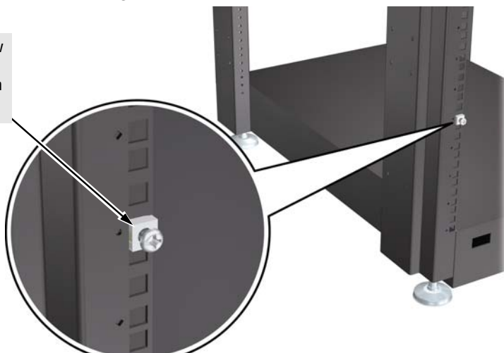
Figure 2-9. Installing the Rack Screw
