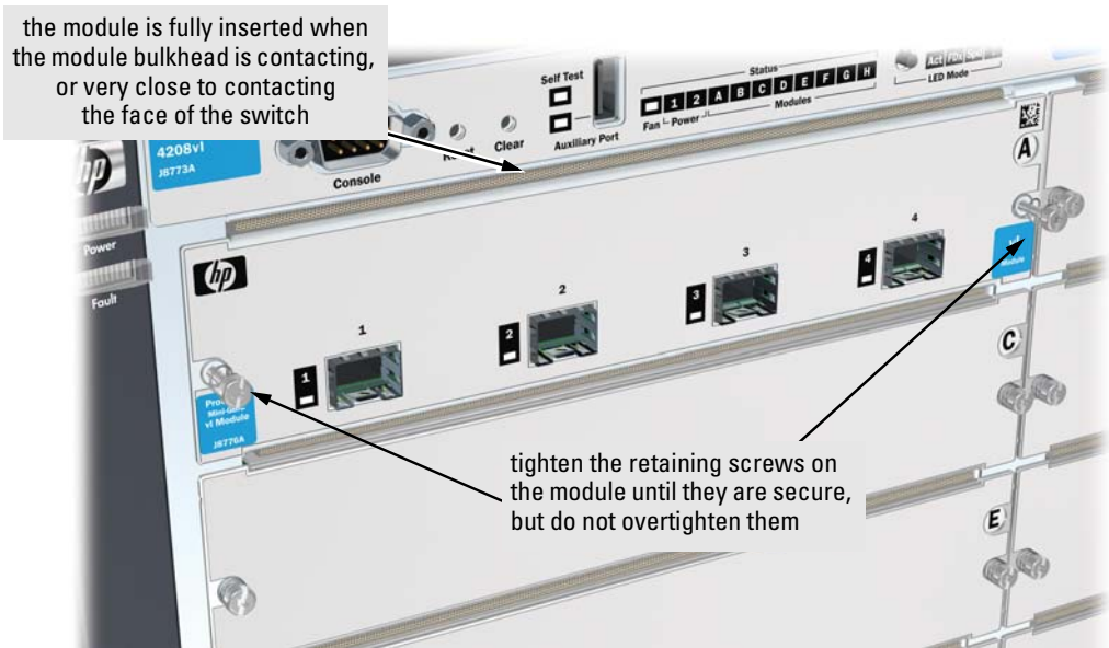
Figure 2-2. Tighten module retaining screws
