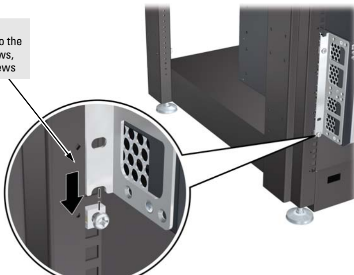
Figure 2-10. Rack mounting using the bracket notch
