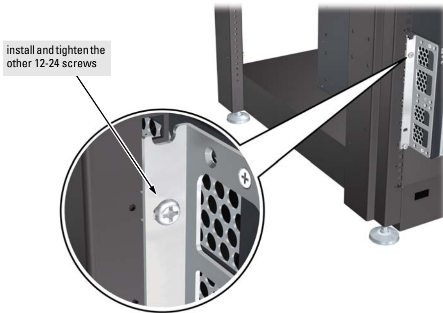
Figure 2-11. Installing final rack mounting screws
