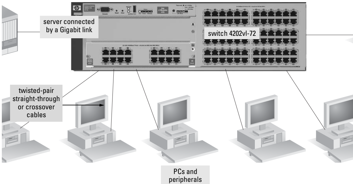
Figure 2-15. Basic Topology
