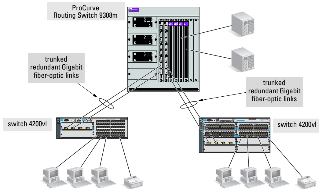
Figure 2-17. Edge Topology
