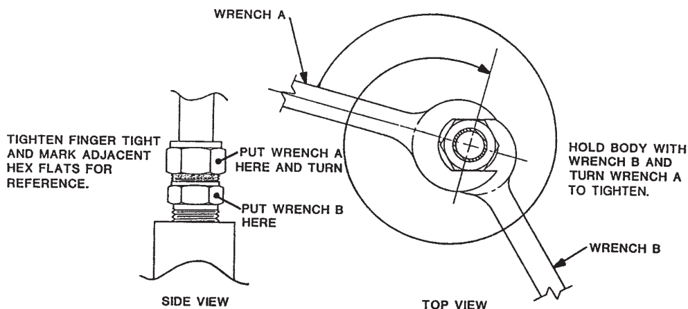
FIGURE 4-2. Male Connector Tightening Diagram
