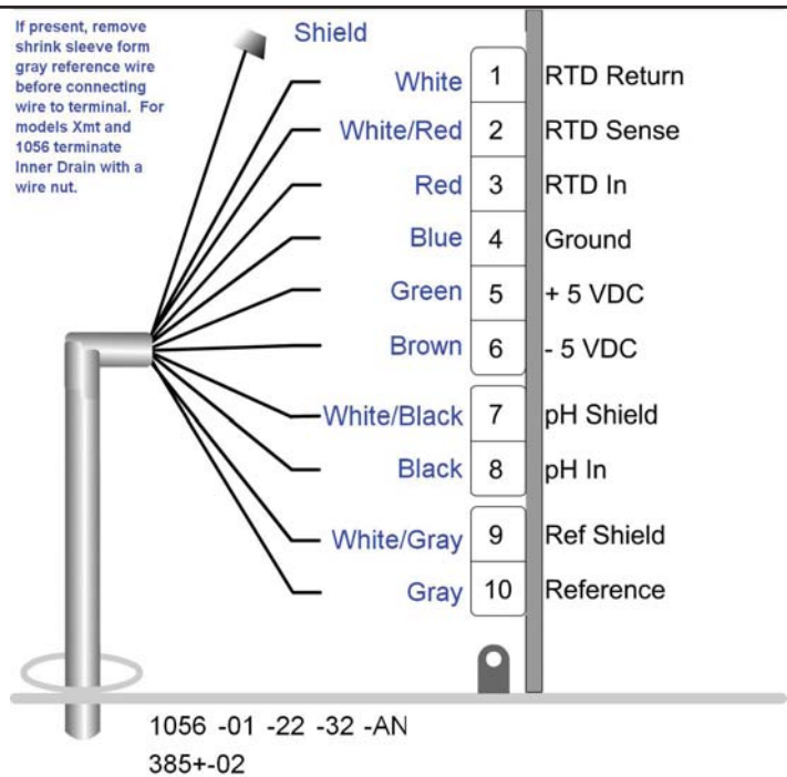
FIGURE 2-11. 5081P-HT VP8 wiring to 385+-04
