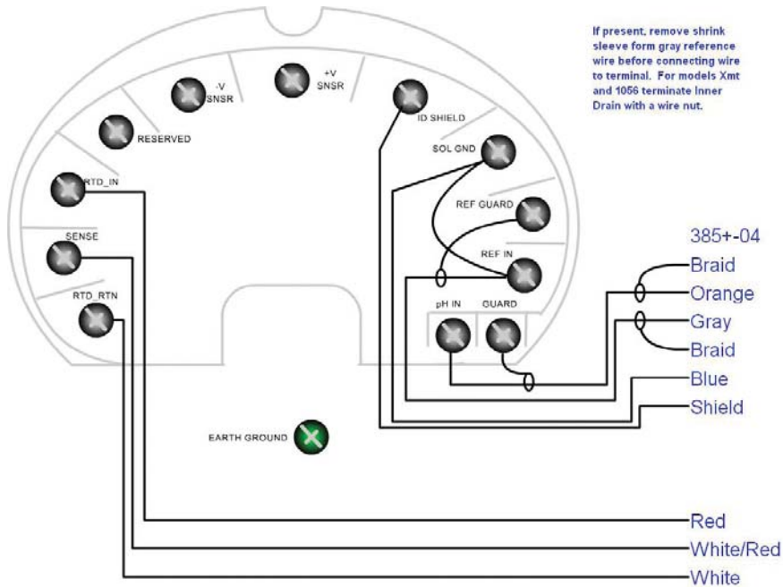
FIGURE 2-8. 6081 VP8 wiring to 385+-04.
