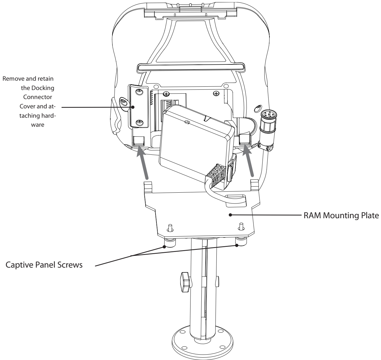
FIGURE 3: RAM MOUNT CABLE ROUTING
