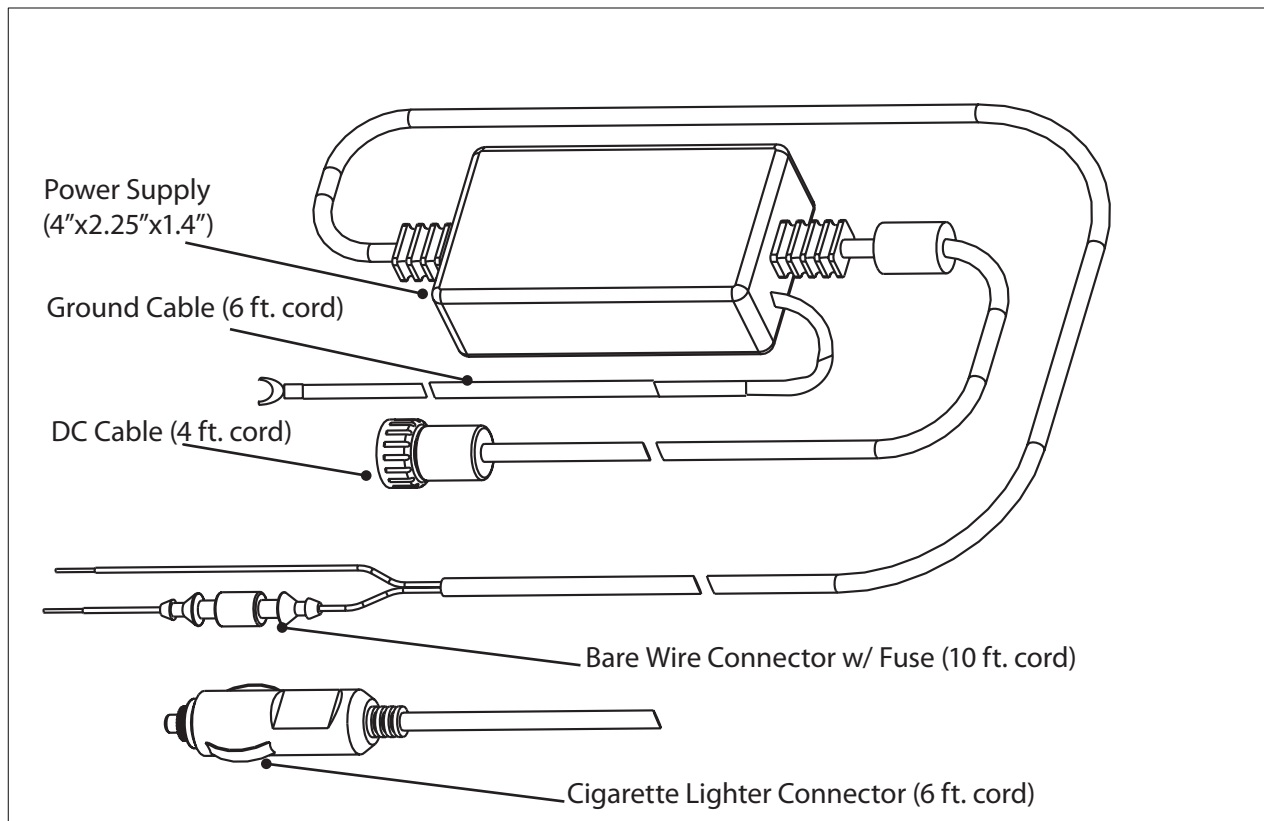
FIGURE 2: POWER SUPPLY VEHICLE CONNECTORS
