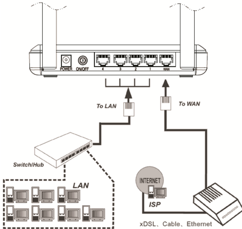
Figure 2-1 Hardware Installation of the PW-RN501D 300Mbps Wireless N Router
