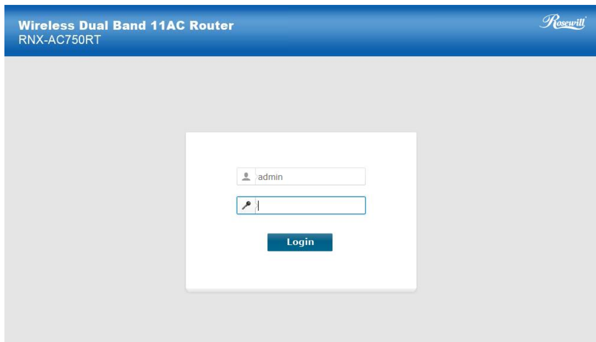
Figure 3-4 Login Windows
