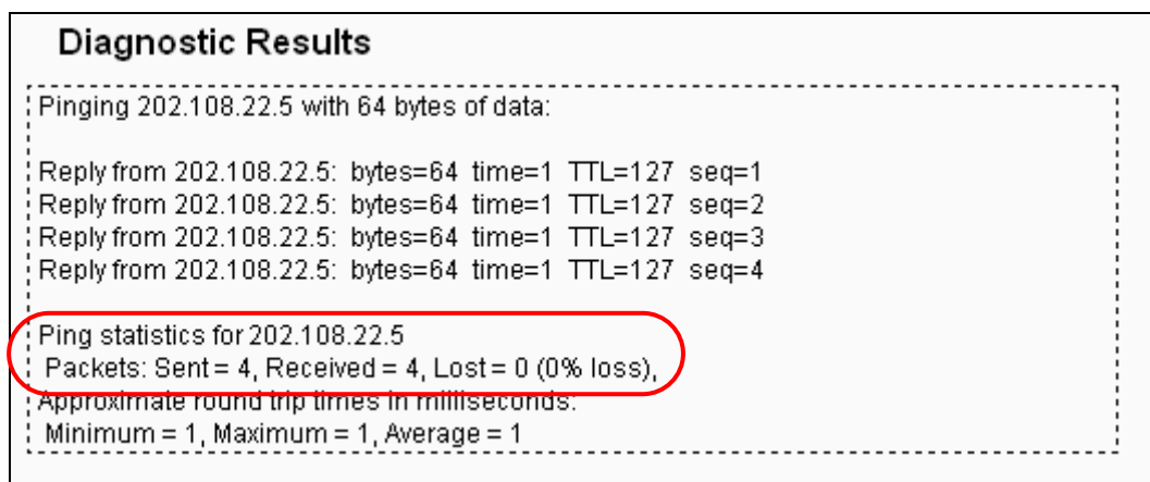
Figure 4-110 Diagnostic Results
