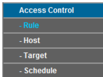
Figure 4-73 Access Control
