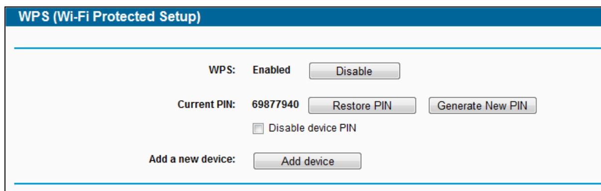
Figure 4-30 WPS
