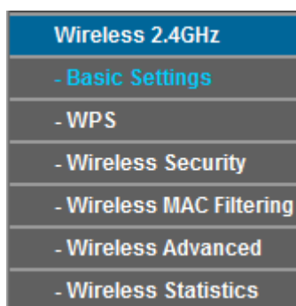
Figure 4-12 Wireless menu
