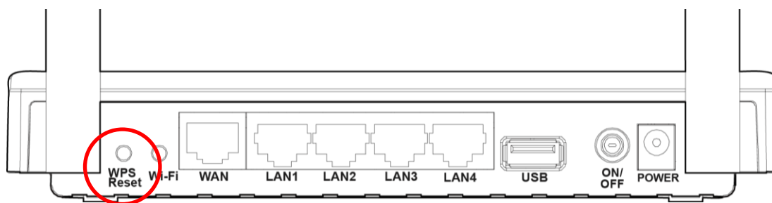
Figure 4-31
