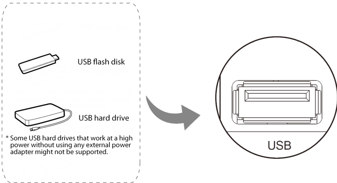
Figure 2-2 USB Installation
