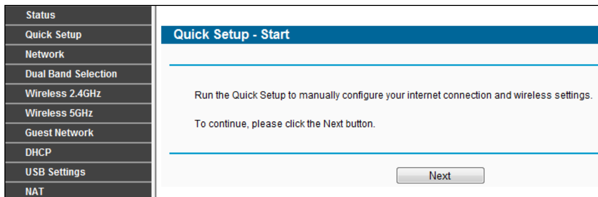
Figure 3-5 Quick Setup
