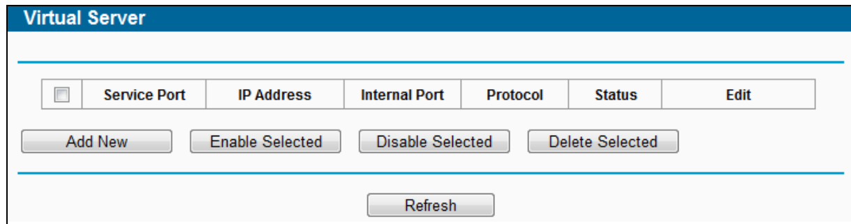
Figure 4-60 Virtual Servers
