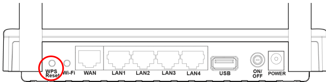
Figure 4-16
