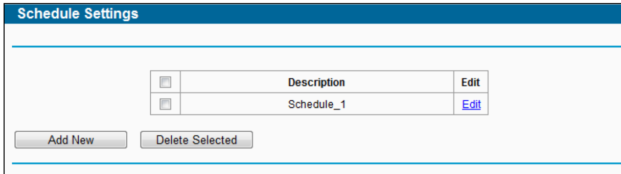
Figure 4-83 Schedule Settings
