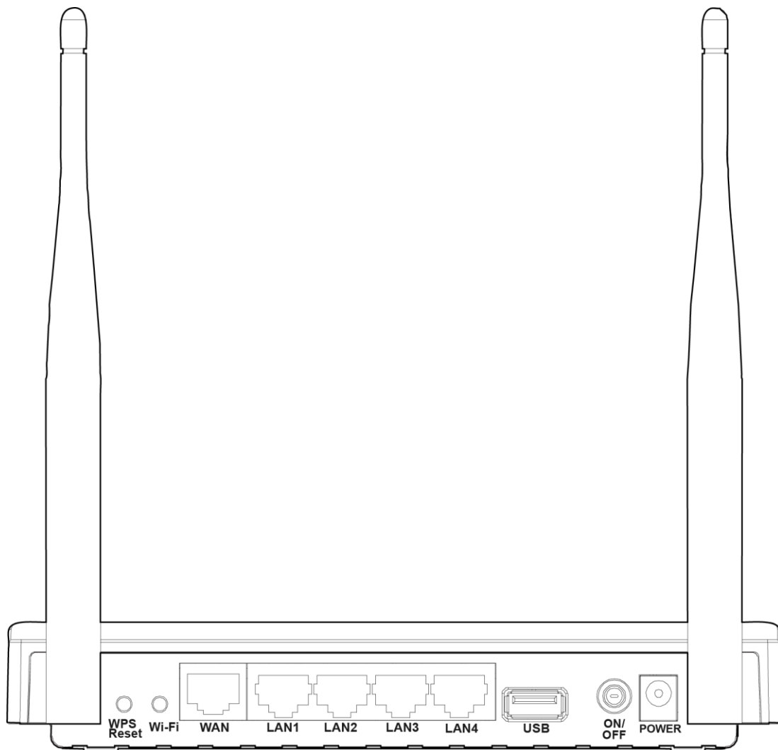
Figure 1-2 Rear Panel sketch
