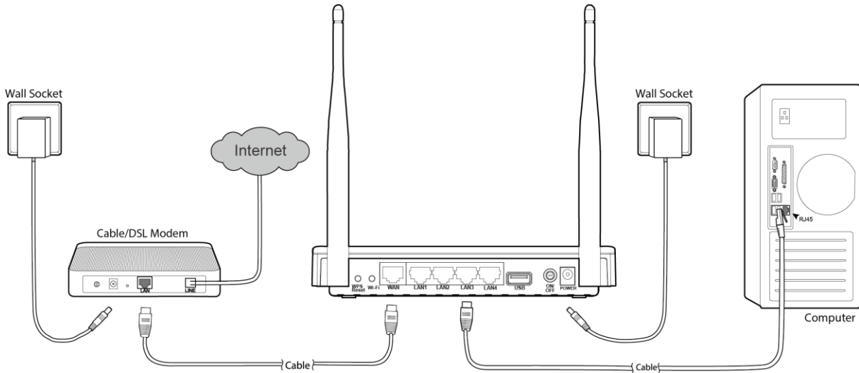
Figure 2-1 Hardware Installation
