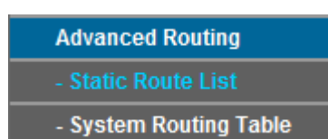
Figure 4-85 Advanced Routing
