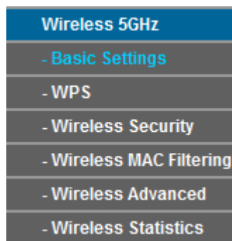
Figure 4-27 Wireless menu
