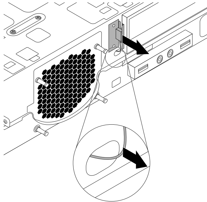
Figure 58. Removing the front Wi-Fi antenna
