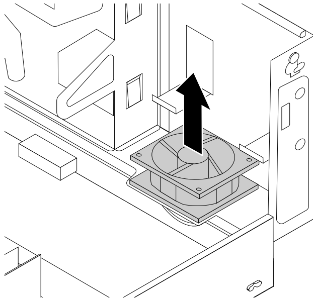
Figure 52. Removing the system fan assembly
