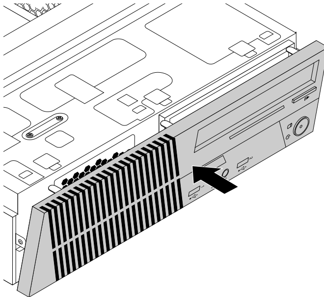
Figure 11. Reinstalling the front bezel
