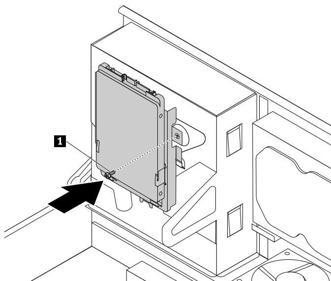
Figure 31. Installing the screw to secure the bracket on the bottom of the optical drive bay
