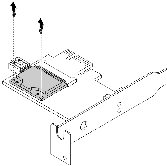
Figure 64. Removing the screws that secure the Wi-Fi card module
