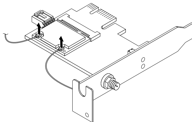
Figure 63. Removing the Wi-Fi antenna cables
