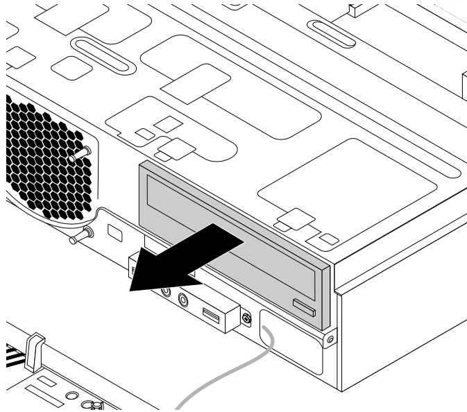
Figure 34. Removing the optical drive
