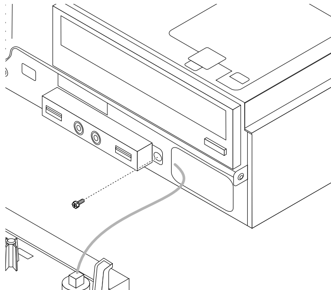
Figure 51. Removing the front audio and USB assembly
