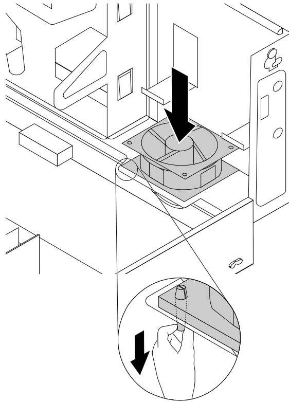
Figure 53. Installing the system fan assembly
