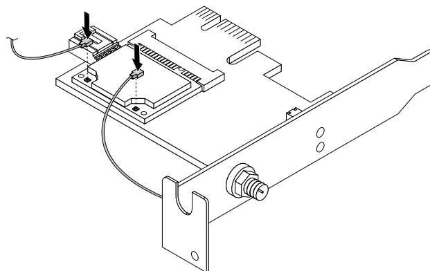
Figure 67. Connecting the Wi-Fi antenna cables
