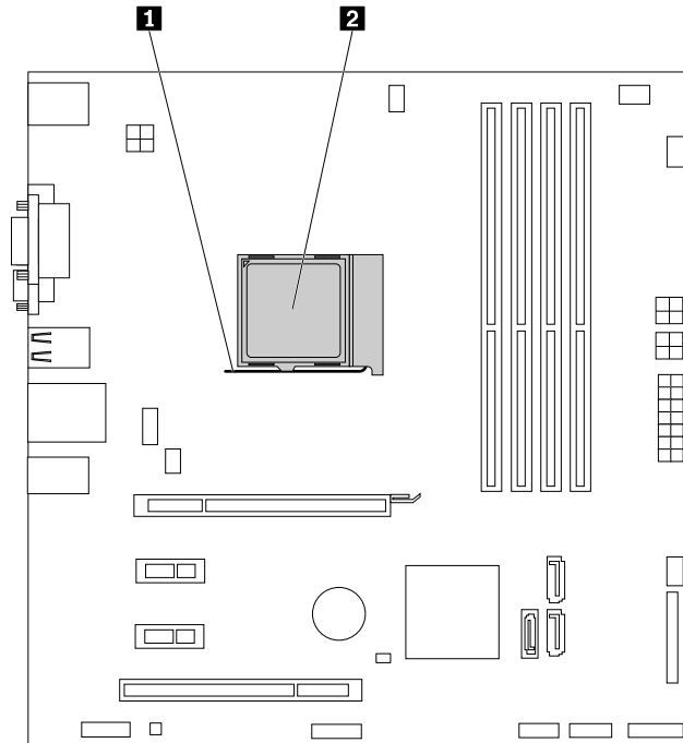
Figure 49. Accessing the microprocessor
