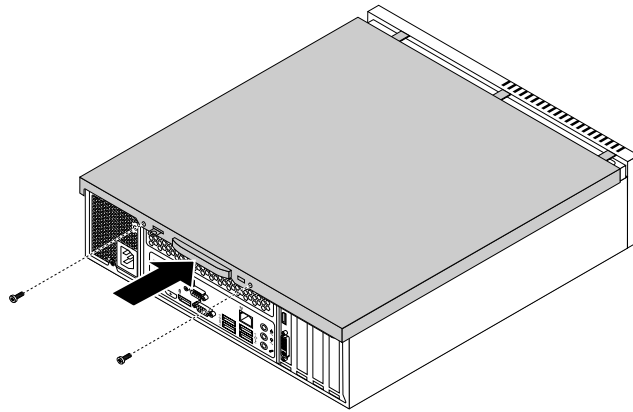
Figure 70. Reinstalling the computer cover
