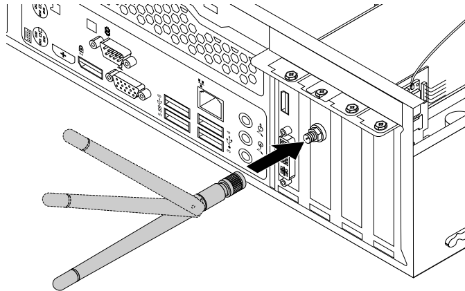
Figure 59. Installing the rear Wi-Fi antenna
