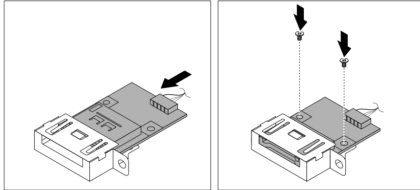
Figure 40. Installing the new slim card reader into the bracket
