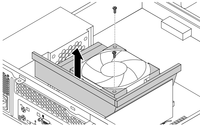
Figure 45. Removing the heat sink fan duct
