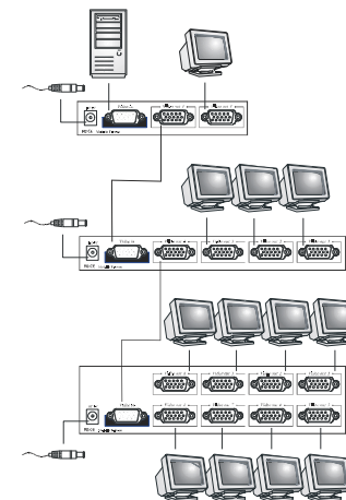
LVS-002E/004E/008E in cascaded application with multiple daisy-chained units
