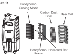
Removing the Carbon Dust Filter*/ Honeycomb Cooling Media:
