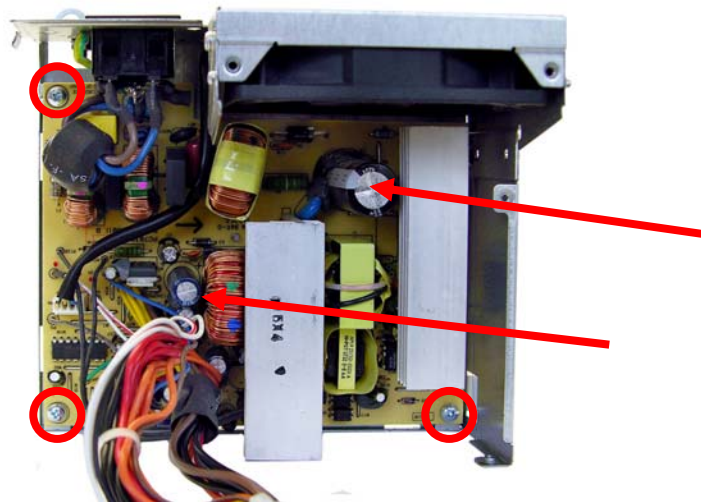
FIGURE 12: POWER SUPPLY 2: PCA screw locations; Capacitors (4) to cut
