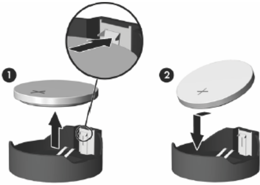
FIGURE 5: Type 3 battery holder
