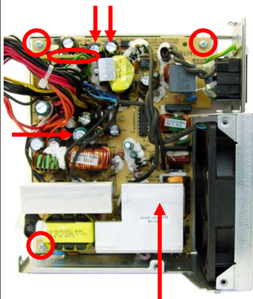
FIGURE 12: POWER SUPPLY 2: PCA screw locations; Capacitors (4) to cut
