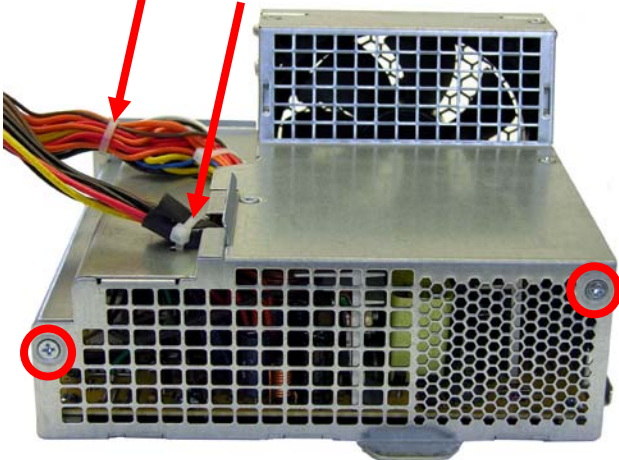
FIGURE 9: Power supply cover screw locations and plastic tie locations
