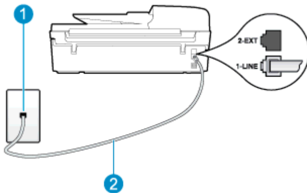
Figure B-1 Back view of the printer
