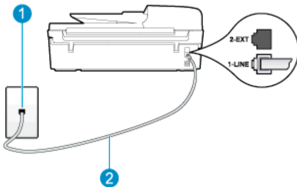
Figure B-5 Back view of the printer
