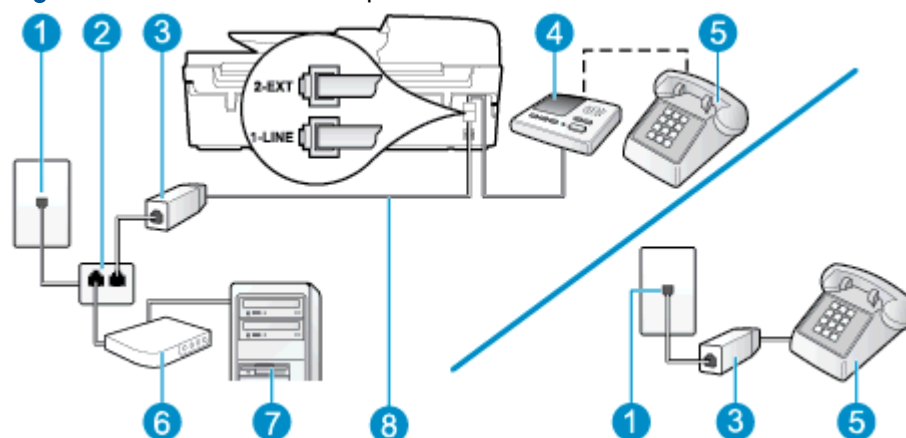
Figure B-15 Back view of the printer
