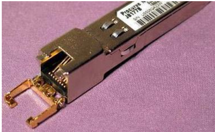
Figure 2. Latch in unlocked position
