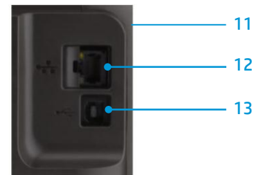
Rear I/O panel close-up
