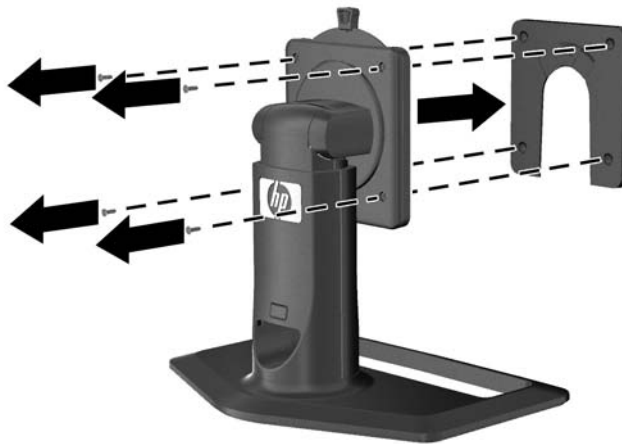
Figure 3-12 Removing the HP Quick Release from the Pedestal Base
