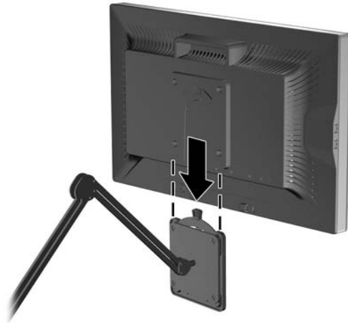
Figure 3-14 Inserting the Monitor Panel into the Quick Release
