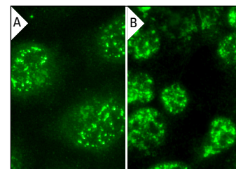
PL6 (C-17): sc-99595. Immunofluorescence staining of methanol-fixed HeLa cells showing nuclear localization (A). Immunofluorescence staining of formalin-fixed Hep G2 cells showing nuclear localization (B).
