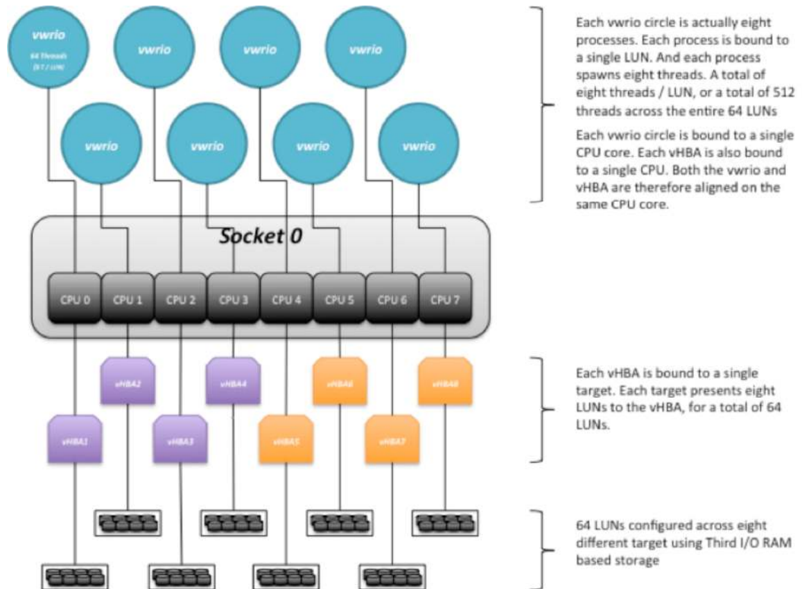
Figure 7. CPU Affinitization
