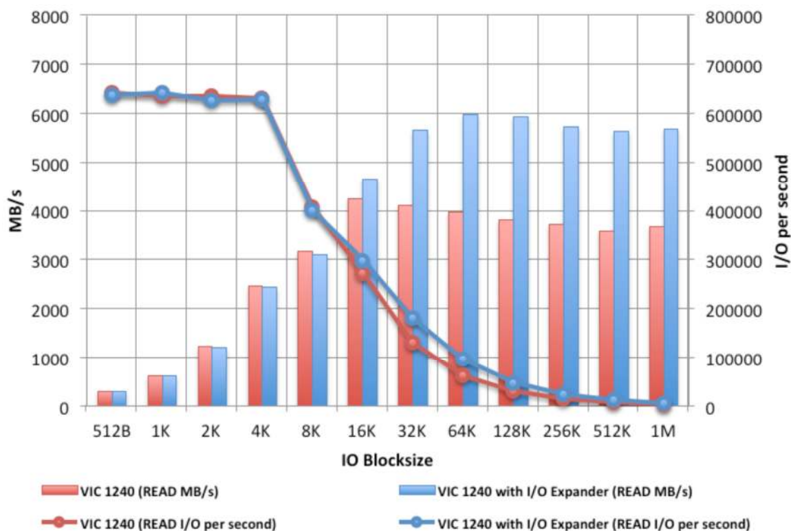
Figure 8. Read Performance
