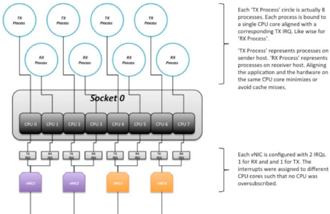
Figure 7. CPU Affinitization
