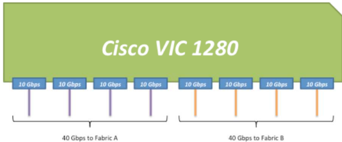
Figure 3. Cisco VIC 1280
