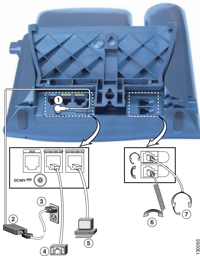
Figure 3-1 Cisco Unified IP Phone 7965G and 7945G Rear Cable Connections
