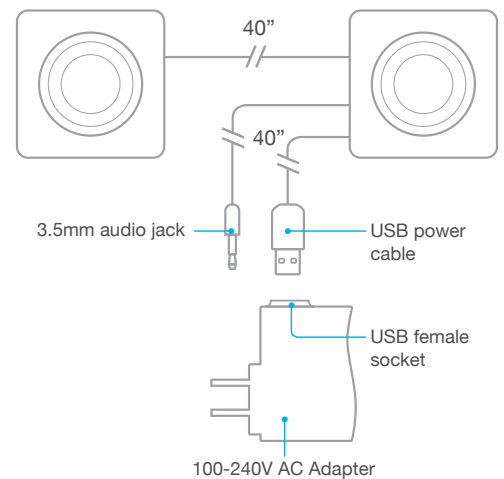
Speaker dimensions: 2"H x 2"W x 2"D
